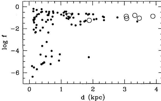
Fig. 1. The molecular fraction f plotted against stellar distance. Solid circles represent Copernicus observations (Savage et al. 1977), while the open circles are from this work. We find that f \sim 0.1 out to large distances in the disk.
