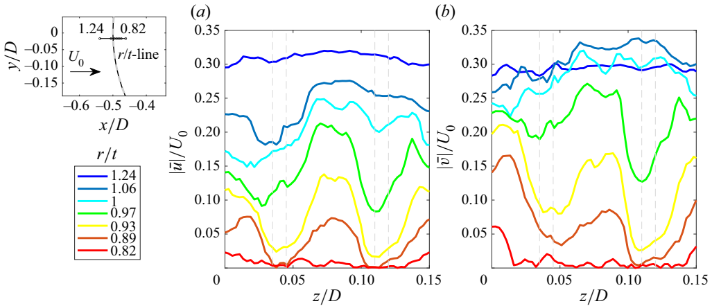
Figure 12. Variation of the flow field along z/D (spanwise direction), approaching and entering the windward side of the SPCC between z/D = 0 and 0.15 : (a) |\bar{u}|/U_0 and (b) |\bar{v}|/U_0 . Each line is represented by an r/t coordinate denoted in the top-left schematic diagram and the narrow area between the grey dashed lines represents the pore structural members.
