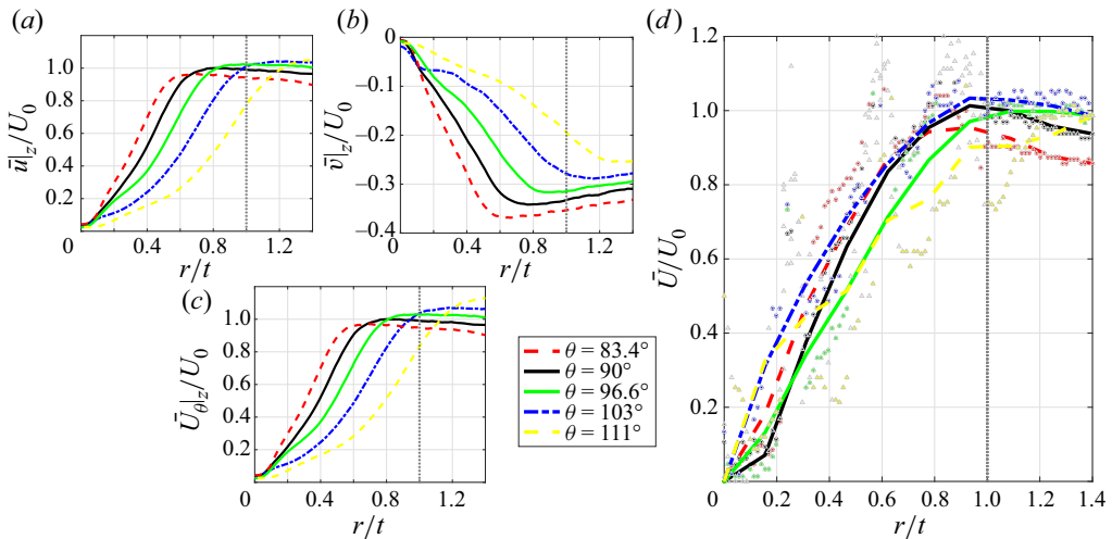
Figure 17. Profiles of flow components recorded along FOV 2 \theta -lines, shown in figure 4: (a) \bar{u}|_z/U_0 , (b) \bar{v}|_z/U_0 , (c) \bar{U}_\theta|_z/U_0 and (d) \bar{U}|_z/U_0 estimated from flow visualisation data in § 3. A vertical dotted line is drawn along r/t = 1 to denote the outer diameter of the SPCC.
