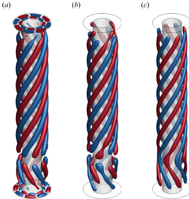
Figure 5. Isosurface of vorticity components for V_E = 500 ; (a) radial vorticity \omega_r = \pm 0.02 , (b) azimuthal vorticity \omega_\varphi = \pm 0.15 , (c) axial vorticity \omega_z = \pm 0.3 .
