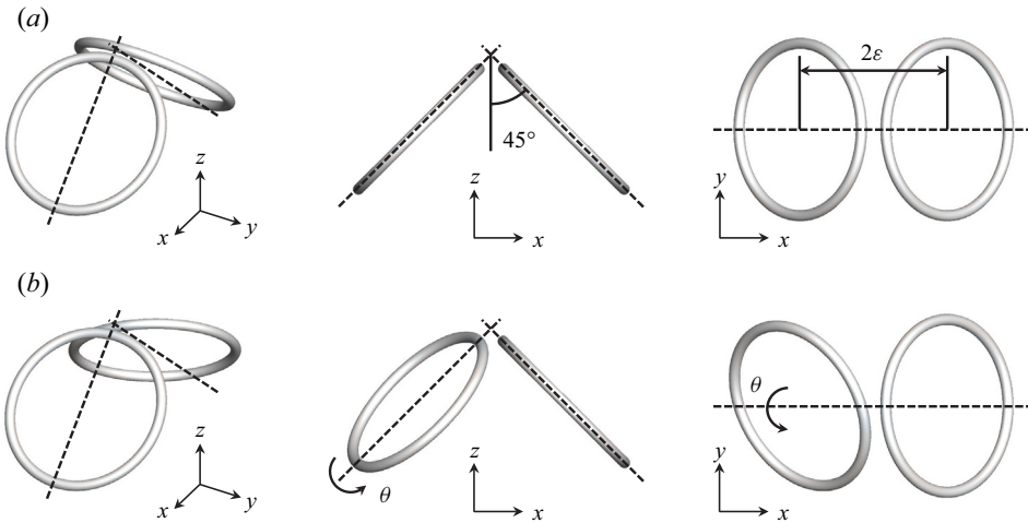
Figure 24. Initial (a) symmetric and (b) asymmetric configurations of a pair of vortex tubes represented by the vorticity isosurface at 4% of maximum initial vorticity.
