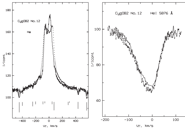
Figure 1. H\alpha (left) and He I 5876 Å (right) profiles in the spectra of Cyg OB2 No. 12 obtained on June 12, 2001 (dotted line) and April 12, 2003 (solid line). The absorption features seen within the H\alpha core correspond to transitions in the line rather than to the telluric spectrum, whose contribution was carefully removed. The vertical dashes show the positions of telluric lines, with the dash lengths proportional to the line strength.
