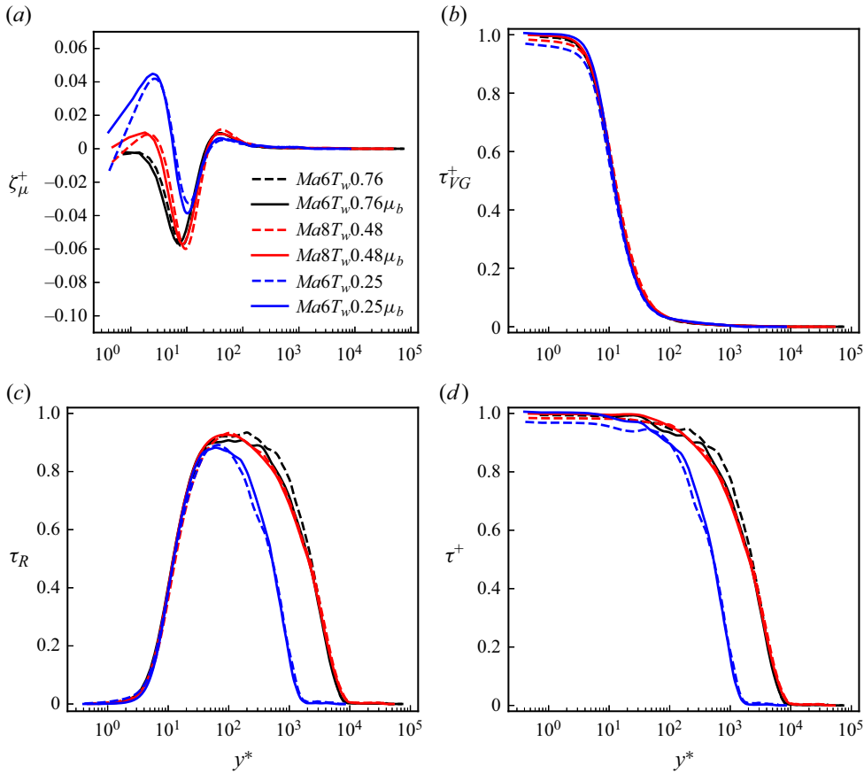
Figure 20. The shear stress budget in the compressible turbulent boundary layer for different cases: (a) viscosity fluctuation term \zeta_{\mu}^+ , (b) generalized viscous shear stress \tau_{VG}^+ = \tau_V^+ + \zeta_{\mu}^+ , (c) Reynolds shear stress \tau_R^+ and (d) total stress \tau^+ along the wall-normal distance in the semi-local scaling.
