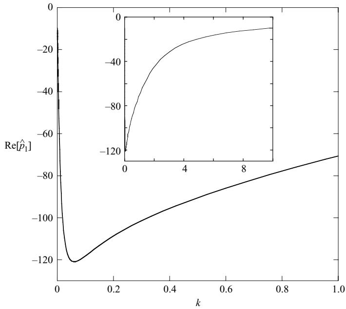
FIGURE C5. The real part of the pressure at the mush–liquid interface \text{Re}[\hat{p}_1(\mathcal{U}_\infty, Pr, k)] versus wavenumber k for \mathcal{U}_\infty = 100 and Pr = 10 . The inset shows the decay at large wavenumber.
