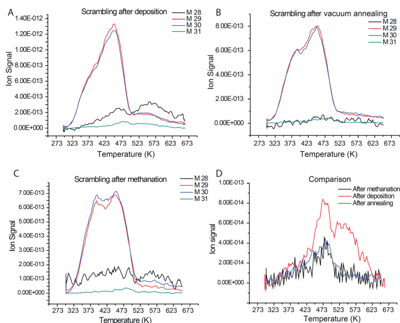
Figure 1. Isotopic CO scrambling TPD spectra after dosing a 1:1 mixture of ^{29}\text{CO} and ^{30}\text{CO} : A) TPD Spectrum collected right after deposition. B) TPD Spectrum collected after sole vacuum annealing. C) TPD Spectrum taken after two methanation runs. D) ^{31}\text{CO} traces magnification, comparing ^{31}\text{CO} spectra in Figure 1A (red), Figure 1B (blue) and Figure 1C (black). The spectra shown here are for experiments performed on 7 nm nanoparticles. Adapted from Masini et al. [5].
