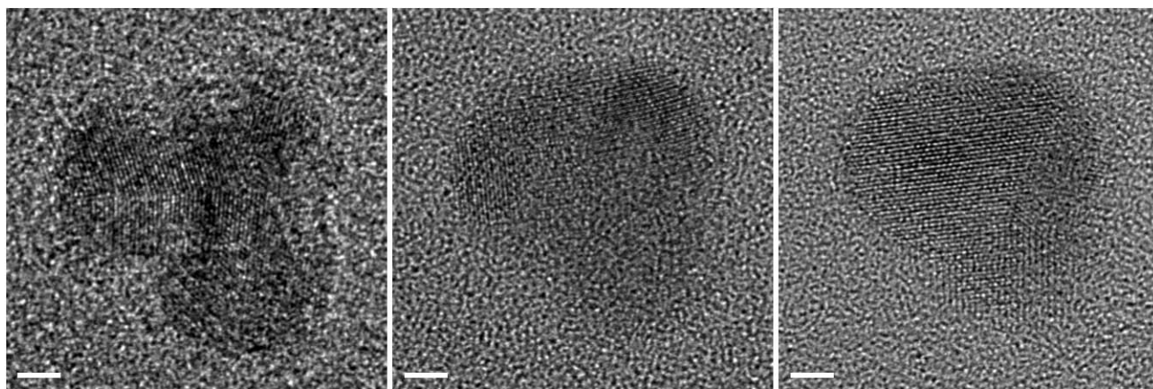
Figure 2. Ruthenium nanoparticle imaged under different conditions relevant for the methanation reaction. Left: Room temperature, vacuum; middle: 427°C, vacuum; right: 427°C 230 Pa 1:10 CO/H 2 .
