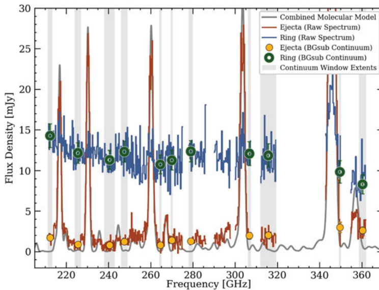
Figure 2. Raw (without background subtraction) band 6–7 spectra and integrated continuum flux densities in the ring and ejecta. Continuum windows selected to be relatively free of emission based on molecular models from Matsuura et al. 2017, accepted .
