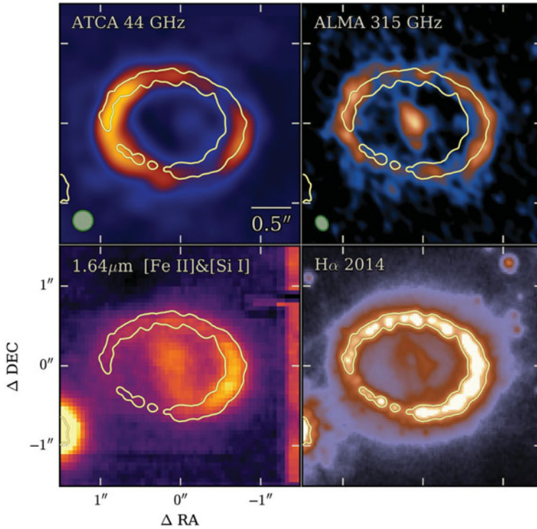
Figure 1. Multi-wavelength view of SN 1987A: ATCA 44 GHz (Zanardo et al. 2013), ALMA 315 GHz (this work), 1.64 \mu\text{m} [Fe II]& [Si I] (Fransson et al. 2016), and \text{H}\alpha (Fransson et al. 2015). The yellow contours trace the optical ring emission.
