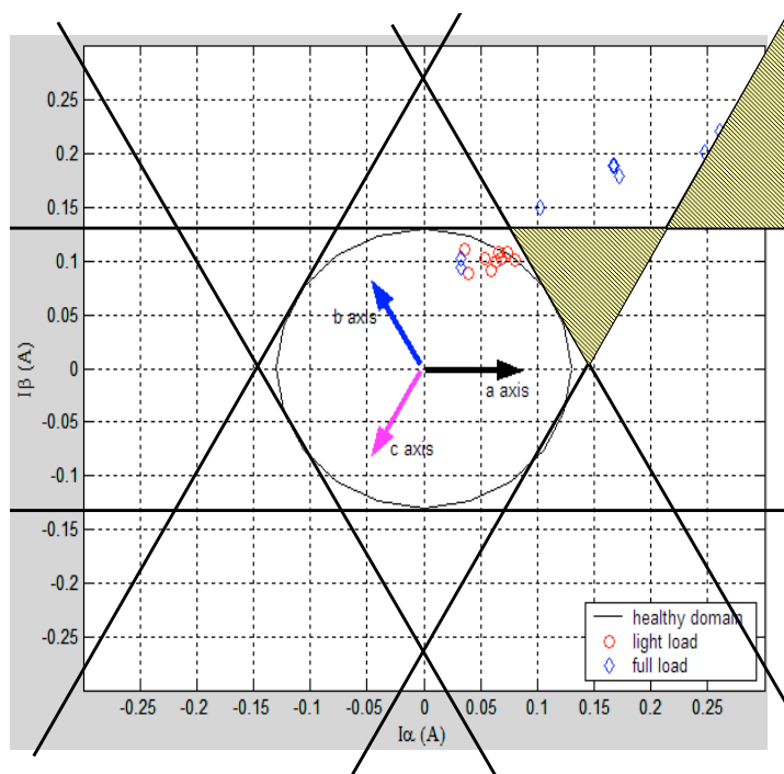
Fig. 5. Concordia mean current vector patterns.
