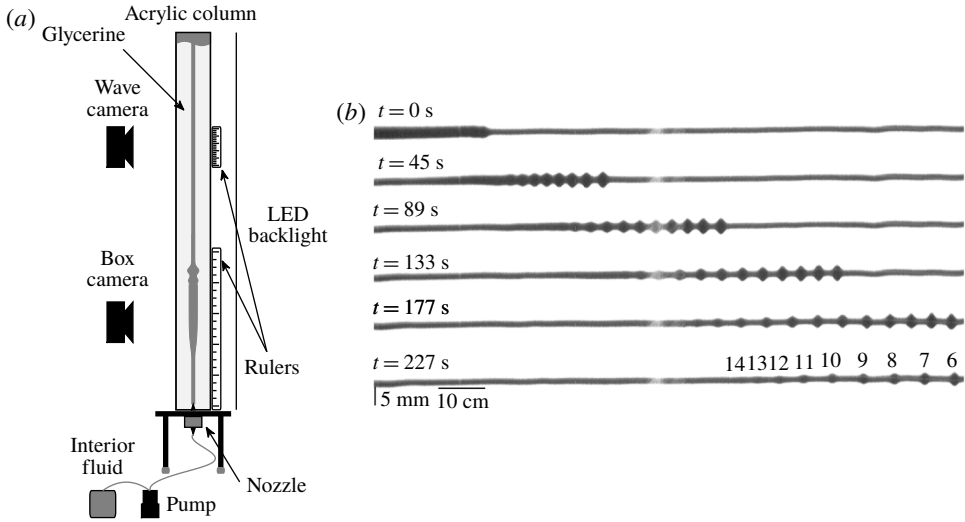
FIGURE 2. (a) Schematic of the experimental apparatus. (b) Box (not entirely shown) with nominal width 25 cm and total height (conduit diameter) 3.2 mm at t = 0 develops into a rank-ordered solitary wavetrain with 12–13 visible solitary waves at t = 177 s. The lead solitary wave (diameter 4.6 mm) propagates on the background conduit with diameter 2.0 mm. At a later time ( t = 227 s) the smallest nine solitary waves – verified by zoomed-in images from the wave camera – are labelled by their amplitude ranking. The 90^\circ clockwise-rotated images exhibit an 8 : 1 aspect ratio. Slight discolouration near the image centre is due to an external scratch. Measured experimental parameters are: \mu^{(i)} = 4.95 \times 10^{-2} Pa s, \mu^{(e)} = 1.0 Pa s, \rho^{(i)} = 1.205 g cm ^{-3} , \rho^{(e)} = 1.262 g cm ^{-3} and Q_0 = 0.25 cm ^3 min ^{-1} . The Poiseuille flow relations (2.1) and (2.2) yield 2R_0 = 2.0 mm and U_0 = 1.35 mm s ^{-1} .
