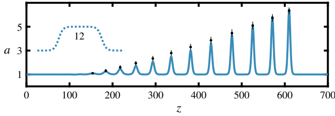
FIGURE 1. An example box initial condition (inset) and its long-time numerical evolution according to the conduit equation (1.1). The number in the inset denotes the predicted number of solitary waves from that initial condition based on the solitary wave resolution method, and the black circles with vertical bars denote the ranges from a quantiled distribution of the predicted solitary wave amplitudes, both derived later in this paper.
