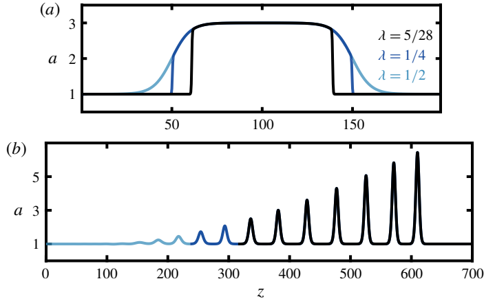
FIGURE 4. (a) Sections of the initial profile from figure 1 for different values of \lambda . The different \lambda sections are identified by colour and shading. (b) Contribution of each \lambda section in terms of the produced solitary waves.
