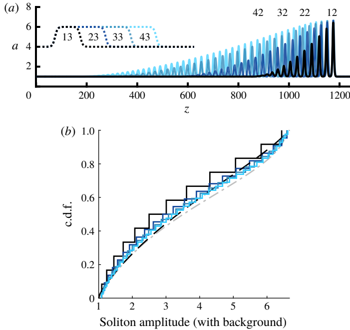
FIGURE 6. (a) Numerical simulations of boxes of different widths and the ensuing solitary waves. Note the evolutions here are at different times and shifted to align so as to better illustrate the similarities and differences in the amplitude distributions. Integers reported above the solitary wavetrains are the number of observed solitary waves to be compared with the prediction (4.10) reported inside the corresponding box initial condition. (b) Observed amplitude distributions (solid) from the same simulations. Predicted amplitude distribution (dashed) from (5.25). Predicted amplitude distribution (dash-dotted) (5.29) for a box.
