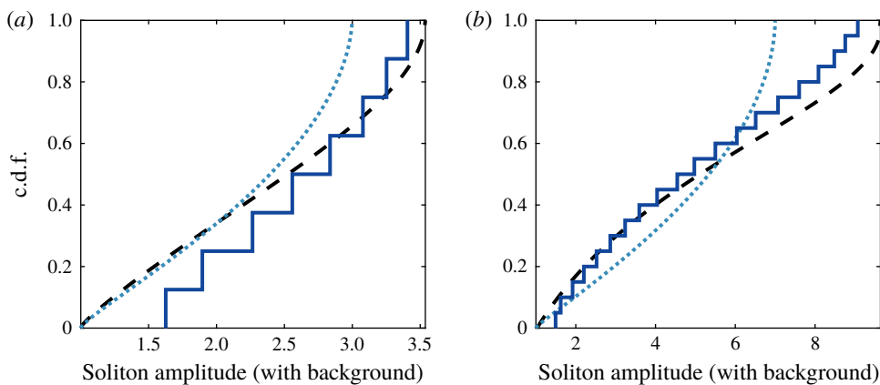
FIGURE 10. Cumulative distribution functions of amplitude distributions from selected experiments (solid line), with the asymptotic prediction from the conduit (dashed line) and KdV (dotted line) equations. Each step in the experimental c.d.f. corresponds to a solitary wave. Box parameters: (a) width = 20 cm ( w = 90 ), a_m = 2 ; and (b) width = 40 cm ( w = 178 ), a_m = 4 .
