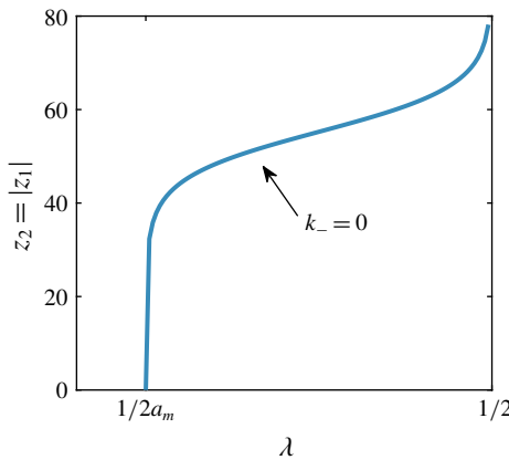
FIGURE 5. Integral endpoints z_{1,2} as a function of the integration constant, \lambda , for the profile in figure 4(a).
