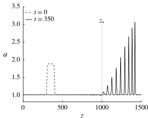
FIGURE 8. Initial (dashed) and final (solid) profiles for a numerical simulation of the conduit equation box problem ( a_m = 0.88 , w = 96 ) that results in nine solitary waves. The location z_* = 1000 separates the solitary wavetrain to the right from small-amplitude dispersive radiation.
