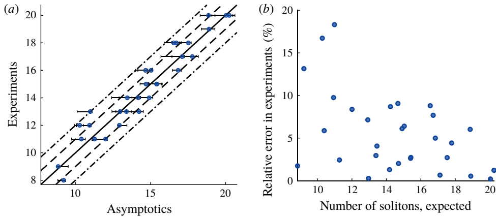
FIGURE 9. (a) Number of solitary waves from experiment (circles) versus the number expected from (4.1). The dashed and dash-dotted lines represent one and two solitary waves away from the expected 1 : 1 relationship. (b) Percentage relative error versus the expected number of solitary waves.
