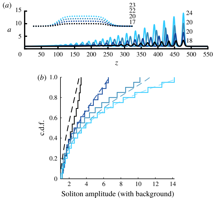
FIGURE 7. (a) Numerical simulations of boxes of different heights and the ensuing solitary waves. The solitary wavetrains are plotted at different times so as to better illustrate the similarities and differences in the amplitude distributions. The expected solitary wave counts (adjacent to the initial profile) and the observed number (adjacent to the solitary wavetrain) do not change much past a certain initial condition amplitude, as expected from (4.13). (b) Amplitude distributions (solid) from the same simulations. Predicted amplitude distribution (dashed) from (5.25).
