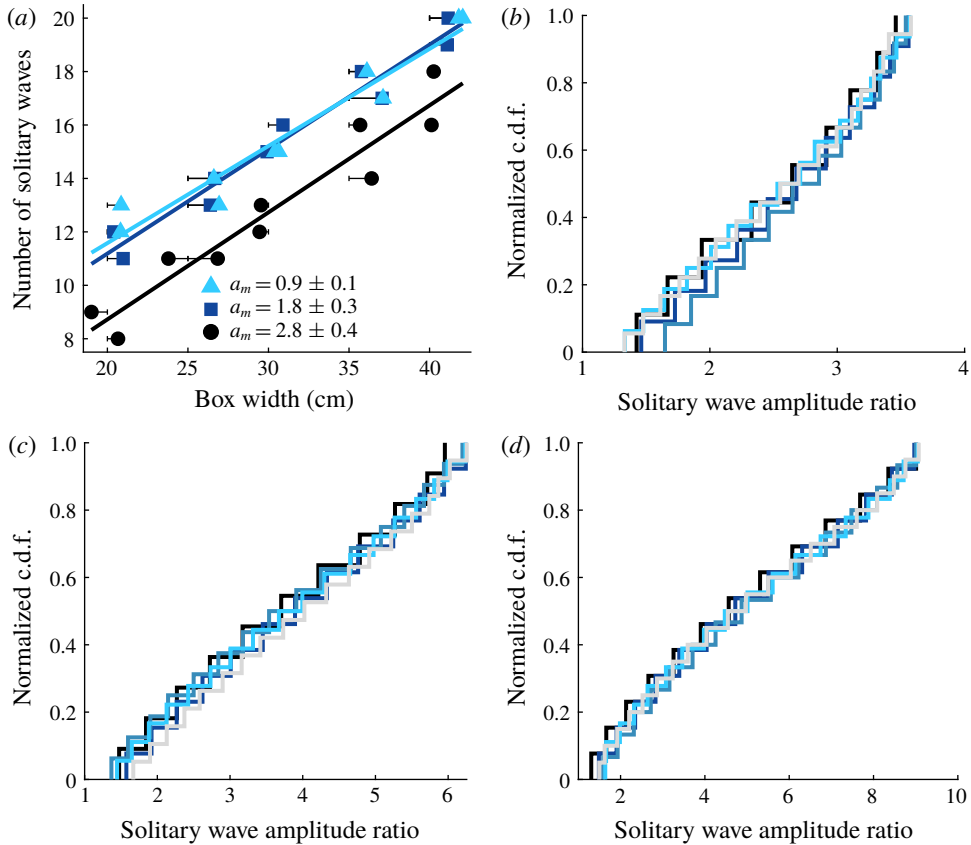
FIGURE 3. (a) Observed number of solitary waves \mathcal{N} as a function of nominal dimensional box width and non-dimensional box height area ratio a_m . Linear fits for fixed box height are included. (b–d) Observed normalised solitary wave c.d.f.s \mathcal{F}(\mathcal{A}) , as defined in (2.4). Panels (b), (c) and (d) correspond to a nominal box height a_m = 1 , a_m = 2 and a_m = 3 , respectively. In each panel, the normalised c.d.f.s for the box widths \{20, 25, 30, 35, 40\} cm are shown, with lighter line styles corresponding to wider boxes.
