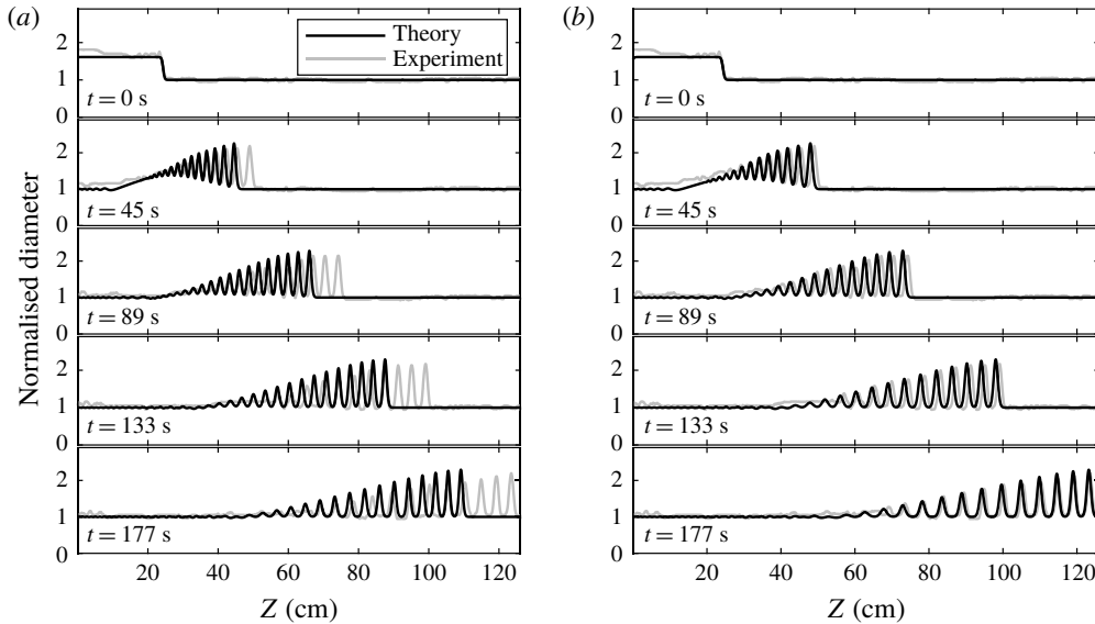
FIGURE 12. Comparison of numerical (dark) and experimental (light) normalised conduit diameter evolution: (a) measured experimental parameters; and (b) fitted experimental parameters. In both panels, the experimental and simulation initial box height a_m = 1.6 is determined from conduit measurements and the experimental initial box width of 25 cm is obtained by the boundary control method (Anderson et al. 2019). The experimental diameter is extracted from images in figure 2(b). (a) Measured nominal experimental parameters in the caption of figure 2 are used to determine the length R_0/\sqrt{8\epsilon} = 1.6 mm and time R_0/(U_0\sqrt{8\epsilon}) = 1.17 s scales, and the non-dimensional box width w = 156 for the numerical simulation. (b) Same as (a) except that the interior and exterior viscosities are fitted, determining the length R_0/\sqrt{8\epsilon} = 1.8 mm and time R_0/(U_0\sqrt{8\epsilon}) = 1.13 s scales, and the non-dimensional box width w = 137 for the numerical simulation.
