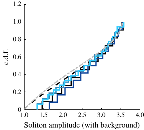
FIGURE 11. Normalised c.d.f.s for solitary wave amplitudes. Experiments (stairs) compare favourably to the predictions from (5.25) for the smoothed box (dashed) and predictions from (5.29) for a pure box (dash-dotted). Colour scale corresponds to initial conditions where a_m = 2 and dimensional widths (light to dark) 25, 30, 35, 40 cm corresponding to non-dimensional widths 112, 134, 156, 178.
