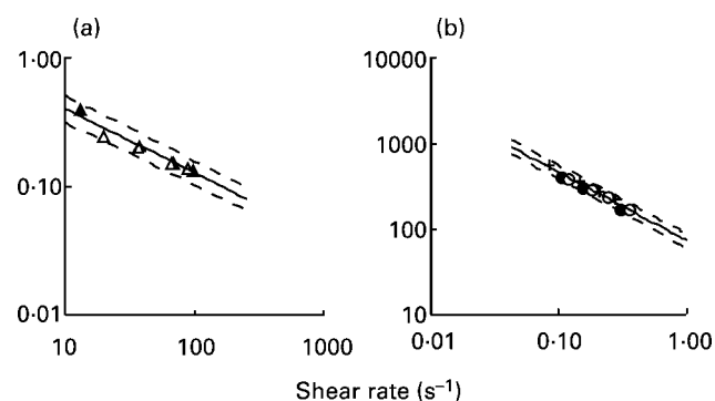
Fig. 2. Coefficient of viscosity v. the shear rate of chicken small intestinal ((a); y = (1.2 \pm 0.2)x ; \Delta , replication 1; \blacktriangle , replication 2) and caecal contents ((b); y = (74 \pm 6)x^{-0.79 \pm 0.04} ); \circ , replication 1; + , replication 2; \bullet , replication 3) at 41^\circ\text{C} . ---, 95% confidence limit for the power regression equation ( P < 0.05 ). The viscosity of these gut contents was measured using the flow behaviour through a glass tube 10 mm in diameter and 1 m long, with 4800, 3800, 2900, and 1900 Pa pressure drops, to measure the viscosity of small intestinal contents, or a tube 21 mm in diameter and 1 m long with 12 000, 11 000, 9700 and 8700 Pa pressure drops to measure the viscosity of caecal contents (logarithmic scale). For details of procedures, see Fig. 1 and p. 868. Note the different scales on the y-axes in the left and right panels.
