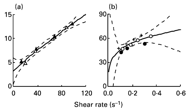
Fig. 3. Shear stress v. against shear rate of chicken small intestinal ((a); y = (0.16 \pm 0.017)x^{0.90 \pm 0.21} + (3.2 \pm 1.1) ; \Delta , replication 1; \blacktriangle , replication 2) and caecal contents ((b), y = (74 \pm 175)x^{0.21 \pm 1.15} ); \circ , replication 1; + , replication 2; \bullet , replication 3). ---, 95% confidence limit for the regression equation ( P < 0.001 ). For details of procedures, see Fig. 1 and p. 868. Note the positive y-intercept of the regression line.
