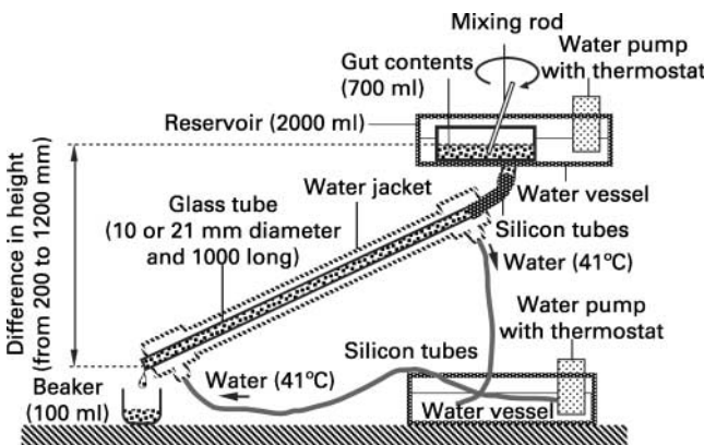
Fig. 1. Tube-flow viscometry for chicken small intestinal and caecal contents.
