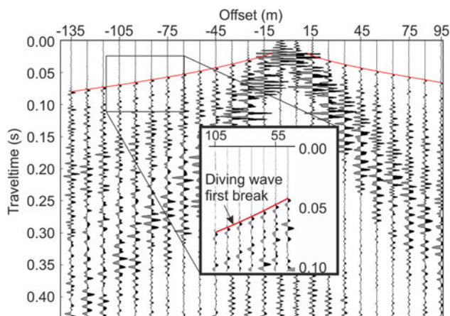
Fig. 2. Pick of the first breaks of the diving waves for the P-wave shot 60 of the parallel profile. Diving wave first arrivals have been picked on cross-correlated data at the zero-crossing of the upgoing part of the Klauder wavelet (red line).
