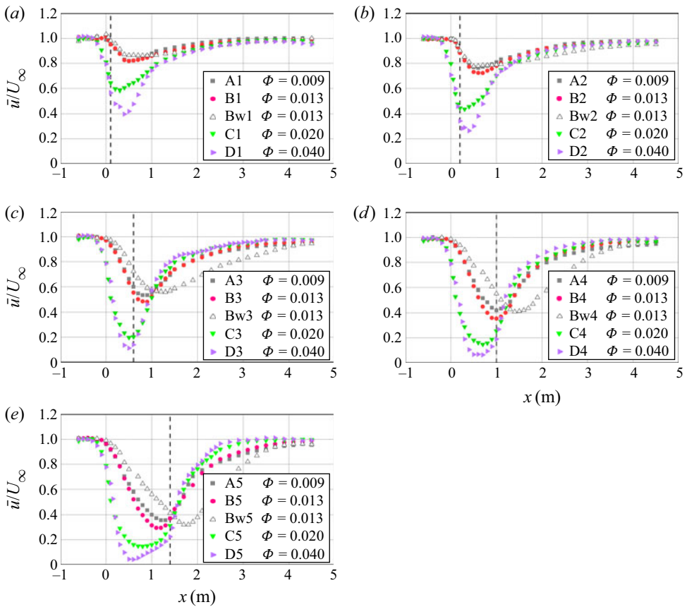
Figure 5. Longitudinal profiles of velocity for patches under the same length: (a) L = 0.1 m, (b) L = 0.2 m, (c) L = 0.6 m, (d) L = 1.0 m, (e) L = 1.40 m. The dashed lines indicate the trailing edges of the patches. The longitudinal velocity is measured at the patch centreline, y = 0 .
