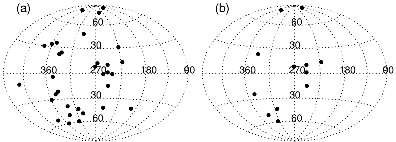
Figure 1 —Distribution in galactic coordinates of SUGAR events with energies above (a) 6 \times 10^{19} eV and (b) 8 \times 10^{19} eV.
