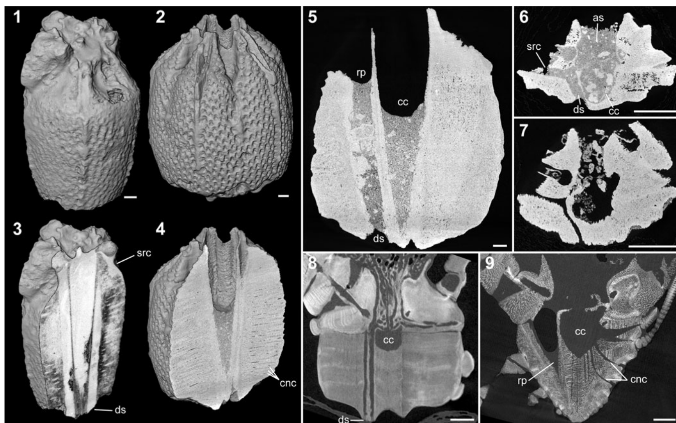
Figure 7. Features of internal anatomy in fossil and extant comatulids as revealed by \mu CT scanning. Scale bar = 1 mm in all images. Scans in (7, 8) taken from Saulsbury (2020). Interradius to right in (5–9). (1) Render of NPL 93001, holotype, Castaneametra hodgesi n. gen. n. sp., oblique view. (2) Render of NPL 103166, paratype, Castaneametra hodgesi n. gen. n. sp., oblique view. (3) Same view as (1), but with the render sliced to show X-ray impedance along a section plane intersecting cirral nerve canals, radial pits, and centrodorsal cavity. (4) Same view as (2) but sliced to show X-ray impedance along a section plane intersecting cirral nerve canals and centrodorsal cavity. (5) NPL 103166, paratype, 2D slice through axis. (6) NPL 103183, holotype, Semiometra alveoradiata n. sp., 2D slice through axis showing configuration of internal cavities. (7) Maastrichtian Semiometra saskiae Jagt, 1999, Maastricht Natural History Museum NHMM K1018a, paratype, 2D slice through axis. (8) Recent Pterometra pulcherrima Clark, 1909a, 2D slice through axis. (9) Recent Notocrinus virilis Mortensen, 1917, 2D slice through axis. as = axial sinus; cc = centrodorsal cavity; cnc = cirral nerve canals; ds = dorsal star; rp = radial pits; src = subradial cleft.
