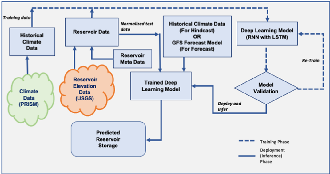
Figure 2. Deep learning-based model schema.
