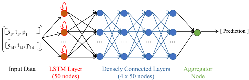
Figure 3. RNN schema. s_n , t_n , and p_n represent reservoir storage, temperature, and precipitation at time step n .
