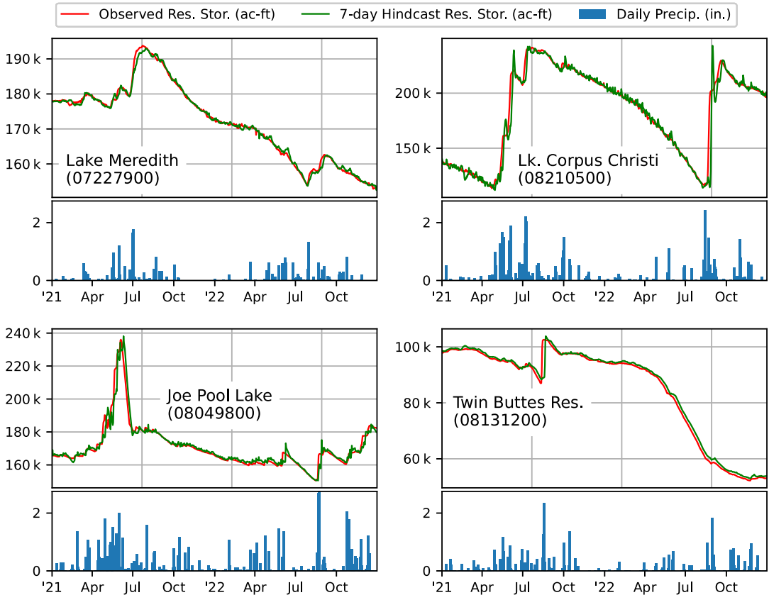
Figure 4. Plots of reservoir storage 7-day hindcast, observed reservoir storage, and observed daily precipitation over the test period.
