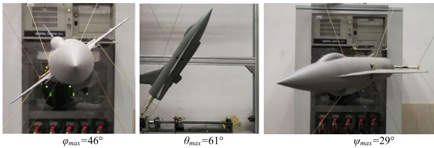
Figure 14. Worspace test of suspension scheme 4.
