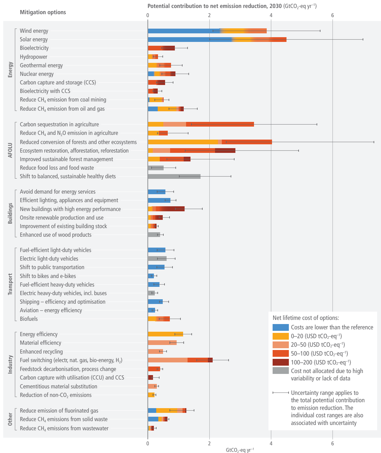
Figure TS.23 | Overview of emission mitigation options and their cost and potential for the year 2030. The mitigation potential of each option is the quantity of net greenhouse gas emission reductions that can be achieved by a given mitigation option relative to specified emission baselines that reflects what would be considered current policies in the period 2015–2019. Mitigation options may overlap or interact and cannot simply be summed together. The potential for each option is broken down into cost categories (see legend). Only monetary costs and revenues are considered. If costs are less than zero, lifetime monetary revenues are higher than lifetime monetary costs. For wind energy, for example, negative cost indicates that the cost is lower than that of fossil-based electricity production. The error bars refer to the total potential for each option. The breakdown into cost categories is subject to uncertainty. Where a smooth colour transition is shown, the breakdown of the potential into cost categories is not well researched, and the colours indicate only into which cost category the potential can predominantly be found in the literature. [Figure SPM.8, 6.4, Table 7.3, Supplementary Material Table 9.SM.2, Supplementary Material Table 9.SM.3, 10.6, 11.4, Figure 11.13, 12.2, Supplementary Material 12.SM.1.2.3]
