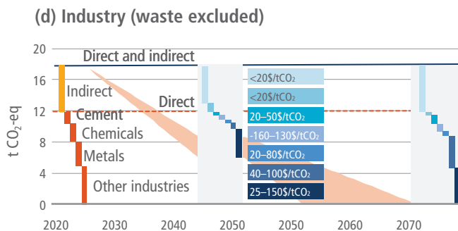
Figure TS.17 | Potentials and costs for zero-carbon mitigation options for industry and basic materials.
