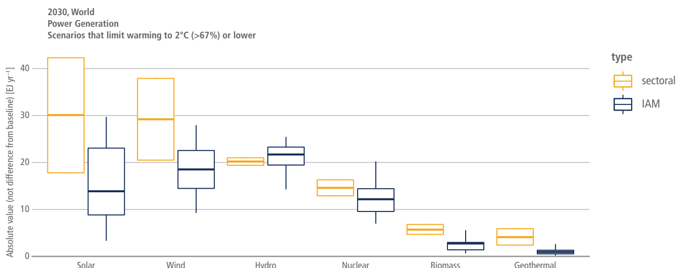
Figure 12.2 | Electricity production in 2030 as calculated by IAMs (dark blue), compared with electricity production potentials found in the sectoral analysis (yellow). Cost cut-offs at USD100 tCO 2 -1 are applied to both electricity production in 2030 as calculated by IAMs and electricity production potentials found in the sectoral analyses. Hinges in the dark-blue box plots represent the interquartile ranges and whiskers extend to the 5th and 95th percentiles, while the hinges in the yellow box plots describe the full range.
