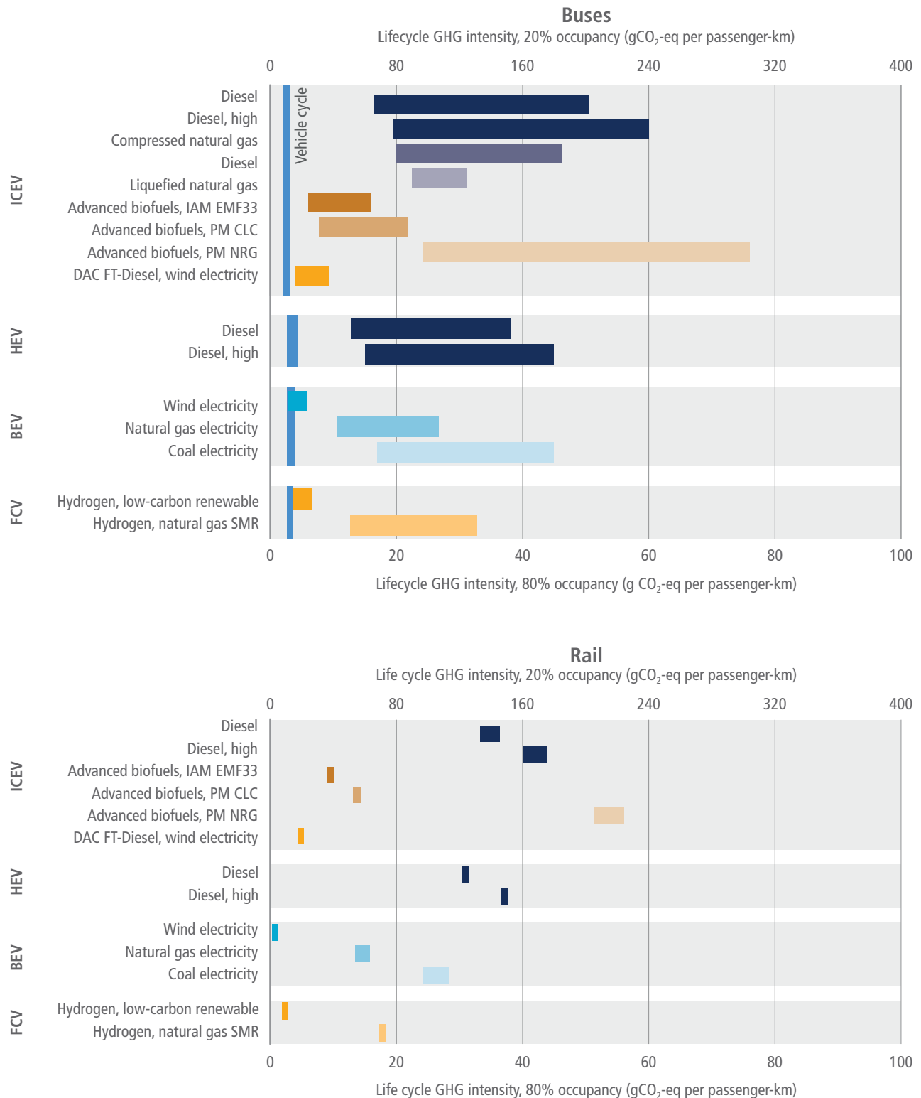
Figure 10.6 | Lifecycle greenhouse gas intensity of land-based bus and rail technologies. Each bar represents the range of the lifecycle estimates, bounded by minimum and maximum energy use per passenger-kilometre, as reported for each fuel/powertrain combination. The ranges are driven by differences in vehicle characteristics and operating efficiency. For energy sources with highly variable upstream emissions, low, medium and/or high representative values are shown as separate rows. The primary x-axis shows lifecycle GHG emissions, in gCO 2 -eq pkm -1 , assuming 80% occupancy; the secondary x-axis assumes 20% occupancy. The values in the figure rely on the 100-year GWP value embedded in the source data, which may differ slightly from the updated 100-year GWP values from WGI. For buses, the main bars show full lifecycle, with vertical bars disaggregating the vehicle cycle. 'Diesel, high' references emissions factors for diesel from oil sands. 'advanced biofuels', refers to the use of second-generation biofuels and their respective conversion and cultivation emissions factors. 'IAM EMF33' refers to emissions factors for advanced biofuels derived from simulation results from the integrated assessment models EMF33 scenarios. 'PM' refers to partial models, where 'CLC' is with constant land cover and 'NRG' is with natural regrowth. 'DAC FT-Diesel, wind electricity' refers to Fischer-Tropsch diesel produced via a CO 2 direct air capture process that uses wind electricity. 'Hydrogen, low-carbon renewable' refers to fuels produced via electrolysis using low-carbon electricity. 'Hydrogen, natural gas SMR' refers to fuels produced via steam methane reforming of natural gas. Results for ICEVs with 'high emissions DAC FT-Diesel from natural gas' are not included here since the lifecycle emissions are estimated to be substantially higher than petroleum diesel ICEVs.
