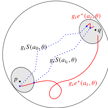
Figure 3. Paths of endpoints (red/solid line) on \partial G = \partial \Gamma and associated near-geodesic sets in \Gamma (blue/dotted) with endpoints in the \epsilon -balls about p and q .
