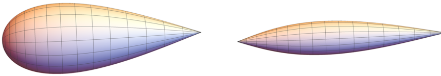
Isometric embeddings of \mathbb{C}\mathbb{P}(3,1) and \mathbb{C}\mathbb{P}(5,3)
