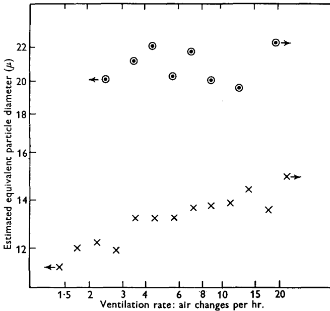
Fig. 1. The relation of ventilation to the size of the air-borne bacterial particles in schoolrooms. ⊙ = Str. salivarius , x = general flora. The arrows indicate that the range of values included in that point extends to include all observed values in the direction of the arrow. The total number of observations was about 1000 for Str. salivarius and 1200 for general flora; the numbers for each point on the graph are not less than 90, or 17 respectively.
