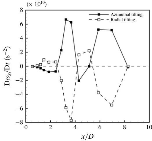
FIGURE 30. Comparison between the azimuthal and radial vortex tilting terms at the liquid surface for case 1; t^* = 11.5 .
