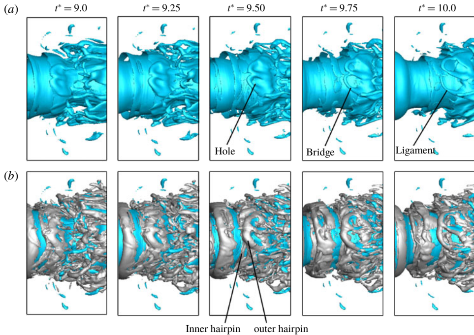
FIGURE 20. (Colour online) Step-by-step tracking of hole formation mechanism in case 1. Liquid surface on a thinning lobe subject to hole formation ( a ); vortex structures indicated by \lambda_2 = -10^{11} \text{ s}^{-2} isosurface on the same frame as ‘ a ’ ( b ). Time is indicated at the top of each column.
