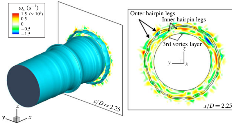
FIGURE 15. (Colour online) Liquid-jet surface and the axial vorticity ( \omega_x ) contours on the plane intersecting the jet at x/D = 2.25 at t^* = 4.5 in case 1.
