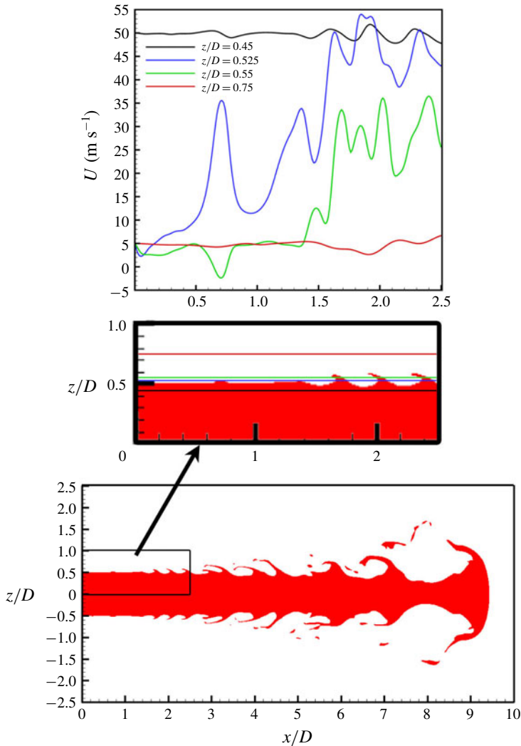
FIGURE 5. (Colour online) Streamwise velocity distribution at different radial distances in the UR near the nozzle exit; case 1, at t^* = 11.25 .
