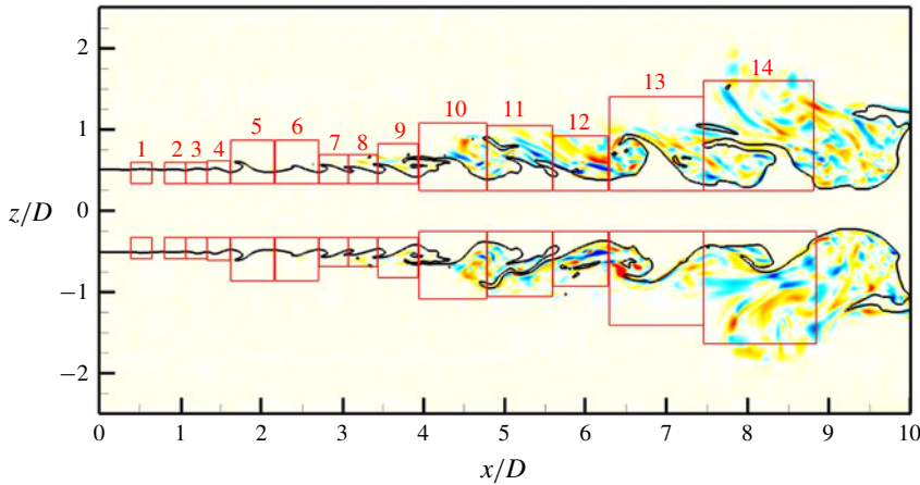
FIGURE 25. (Colour online) Identification of the control volumes used for calculation of vorticity components per KH wavelength.
