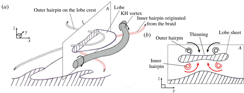
FIGURE 16. (Colour online) Three-dimensional schematics showing the overlapping of the two hairpin vortices – one from the lobe crest (outer black tube, pointing downstream), and the other from the braid (inner red tube, pointing upstream) (a); A is the plane in which (b) is drawn; cross-sectional view of the A-plane, showing the thinning of the lobe sheet due to the combined induction of the two oppositely orientated overlapping hairpins (b). The vortex schematics are periodic in x - and y -directions (ZSH2).
