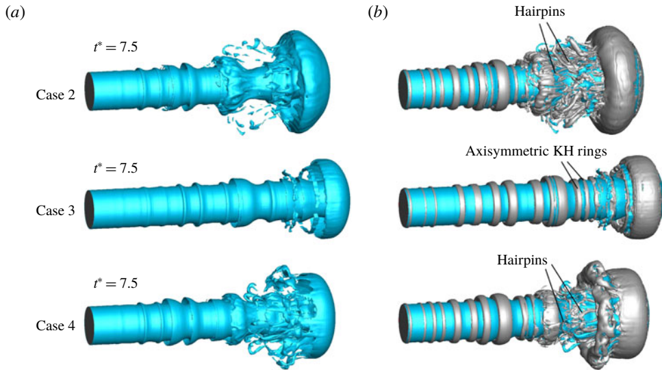
FIGURE 38. (Colour online) Liquid-jet surfaces (a), and the vortex structures (b) in case 2 (top), case 3 (centre) and case 4 (bottom); t^* = 7.5 .
