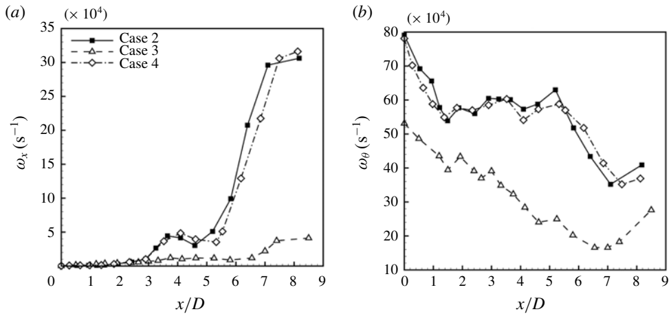
FIGURE 36. Axial distribution of \omega_x (a) and \omega_\theta (b) for cases 2, 3 and 4, at t^* = 11.5 .
