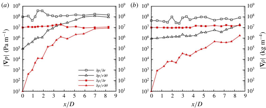
FIGURE 33. (Colour online) Comparison between the radial and azimuthal pressure gradients and density gradients in case 1 (a) and case 3 (b), t^* = 11.5 .
