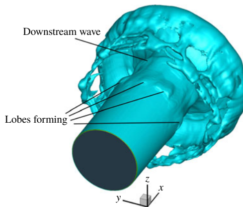
FIGURE 12. (Colour online) Liquid jet surface at t^* = 3.5 in case 2.
