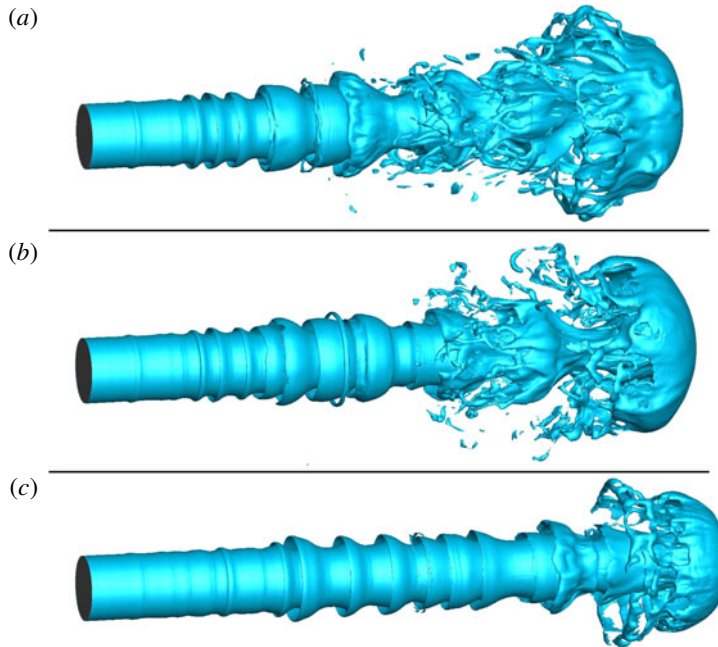
FIGURE 9. (Colour online) Liquid-jet surface for case 1 (a); case 2 (b); and case 3 (c) at t^* = 11.25 .
