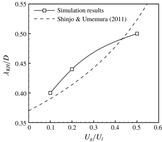
FIGURE 6. Average KH wavelength for different velocity ratios for a constant U_l .
