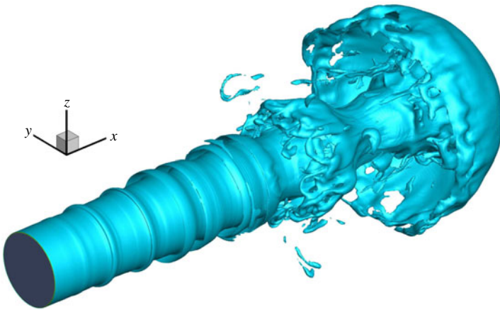
FIGURE 19. (Colour online) Liquid-jet surface at t^* = 8.5 in case 1.
