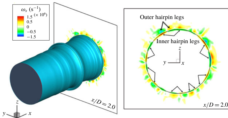
FIGURE 14. (Colour online) Liquid-jet surface and the axial vorticity ( \omega_x ) contours on the plane intersecting the jet at x/D = 2.0 at t^* = 4.5 in case 1.
