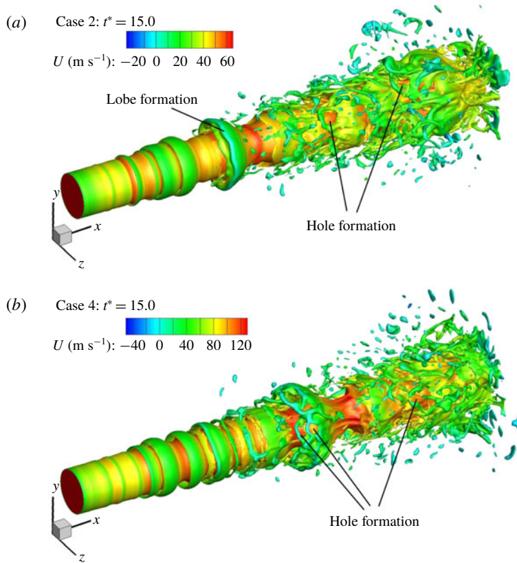
FIGURE 39. (Colour online) Comparison of the liquid-jet surface in case 2 (a) and case 4 (b) at t^* = 15 . The liquid surfaces are coloured with streamwise velocity contours.
