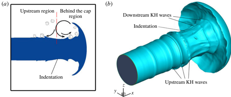
FIGURE 3. (Colour online) Schematic of vortex regions and wave transmission paths (a). Liquid-jet surface showing different instability types and their propagation directions in case 1 (b).
