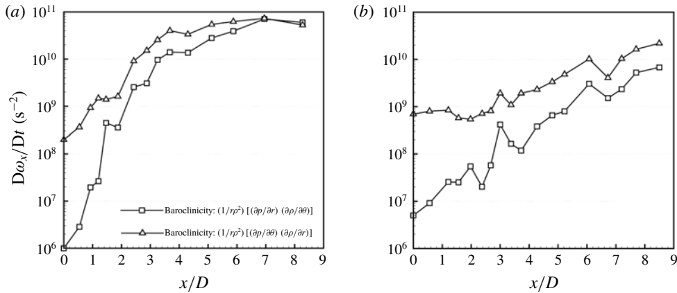
FIGURE 32. Comparison between the radial and azimuthal pressure gradient terms of baroclinicity in case 1 (a) and case 3 (b), t^* = 11.5 .
