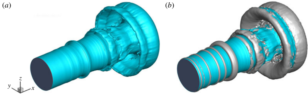
FIGURE 13. (Colour online) Liquid-jet surface (a); and vortex structures indicated by \lambda_2 = -10^{11} \text{ s}^{-2} isosurface (b) at t^* = 4.5 in case 1.
