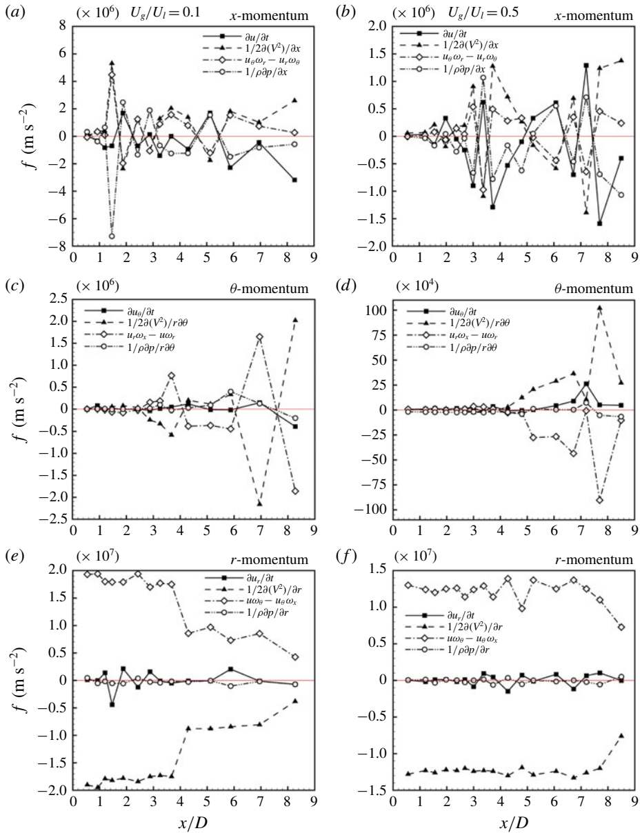
FIGURE 34. (Colour online) Comparison of the terms in the axial momentum equation (a,b), azimuthal momentum equation (c,d) and radial momentum equation (e,f), for case 1 (a,c,e) and case 3 (b,d,f); t^* = 11.5 .
