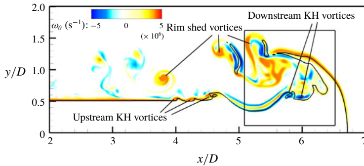
FIGURE 4. (Colour online) Azimuthal vorticity ( \omega_\theta ) contours showing vortices near the interface – case 1.
