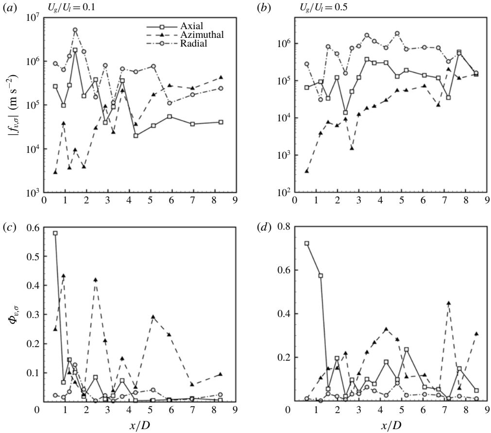
FIGURE 35. Comparison of viscous and surface tension forces, |f_{v,\sigma}| (a,b), and normalized viscous and surface tension forces, \Phi_{v,\sigma} (c,d), for case 1 (a,c) and case 3 (b,d), t^* = 11.5 .
