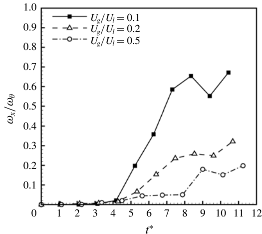
FIGURE 24. Kinematic variation of \omega_x/\omega_\theta for different velocity ratios.
