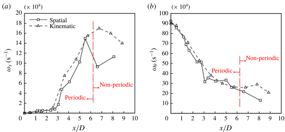
FIGURE 26. (Colour online) Comparison of the spatial and kinematic calculations of \omega_x (a); and \omega_\theta (b) in case 1 ( \hat{U} = 0.1 ).
