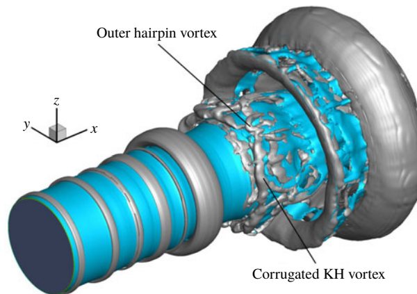
FIGURE 17. (Colour online) Liquid-jet surface (blue) and vortex structures (grey) at t^* = 5.0 in case 1.
