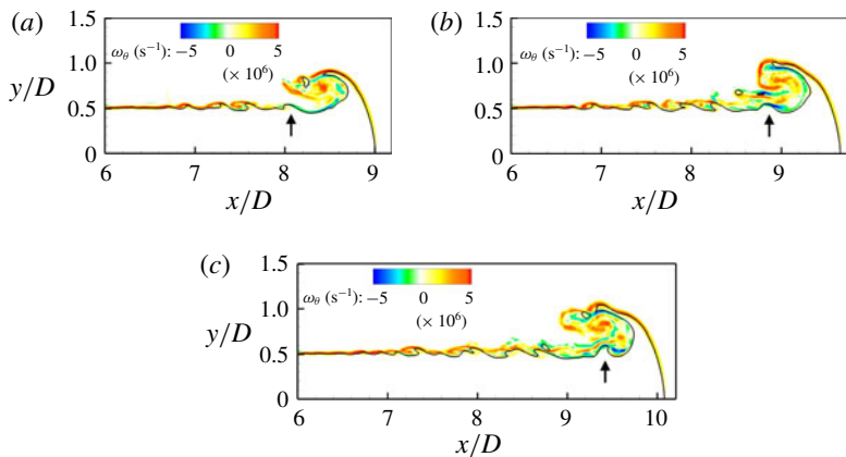
FIGURE 10. (Colour online) Change in the roll-up direction of the KH wave as it moves from the UR to the BCR region in case 2, at t^* = 10.5 (a); t^* = 11.0 (b); and t^* = 11.5 (c).
