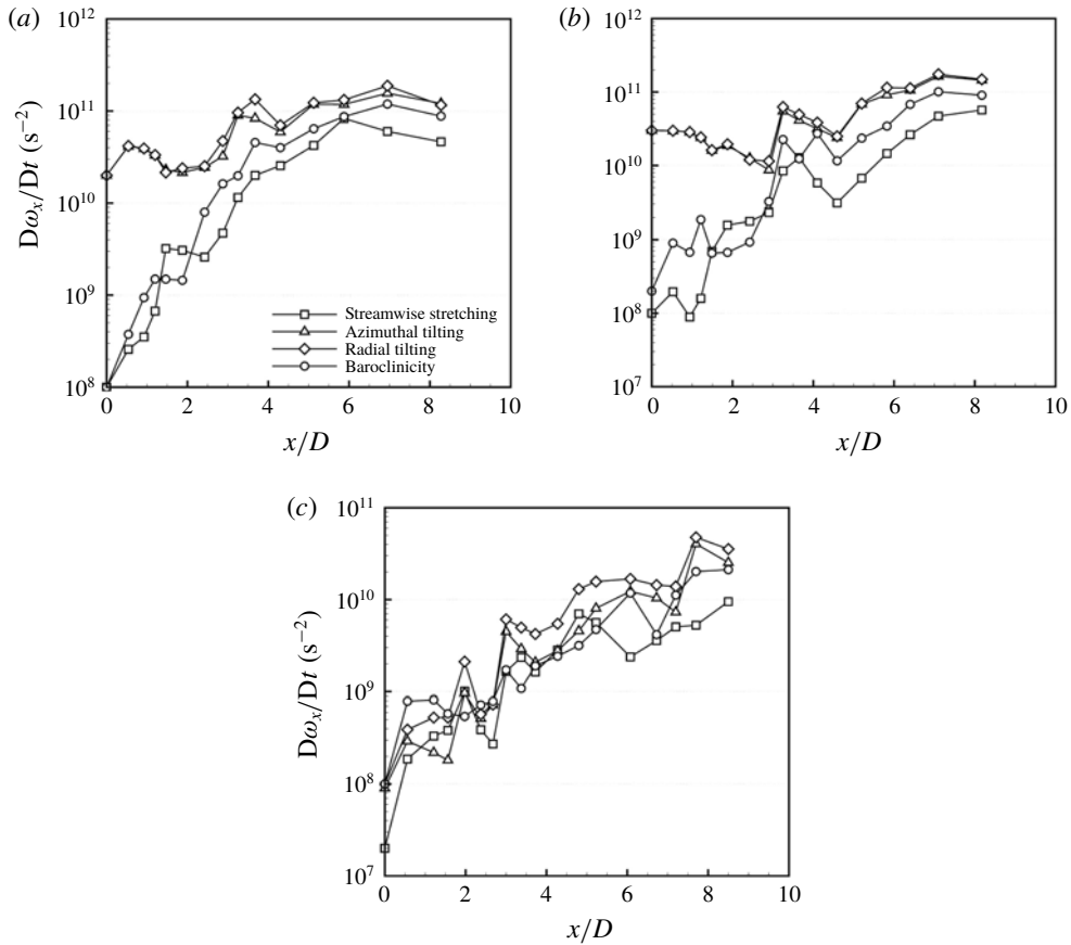
FIGURE 29. Contributions of streamwise vortex stretching (squares), azimuthal vortex tilting (triangles), radial vortex tilting (diamonds), and baroclinicity (circles) to the generation of \omega_x at the liquid surface for case 1 (a) case 2 (b) and case 3 (c); r^* = 11.5 .
