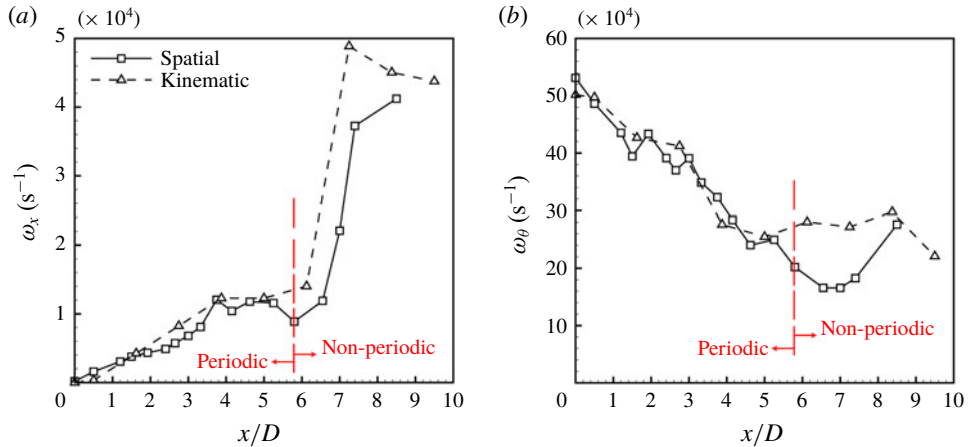
FIGURE 27. (Colour online) Comparison of the spatial and kinematic calculations of \omega_x (a); and \omega_\theta (b) in case 3 ( \hat{U} = 0.5 ).
