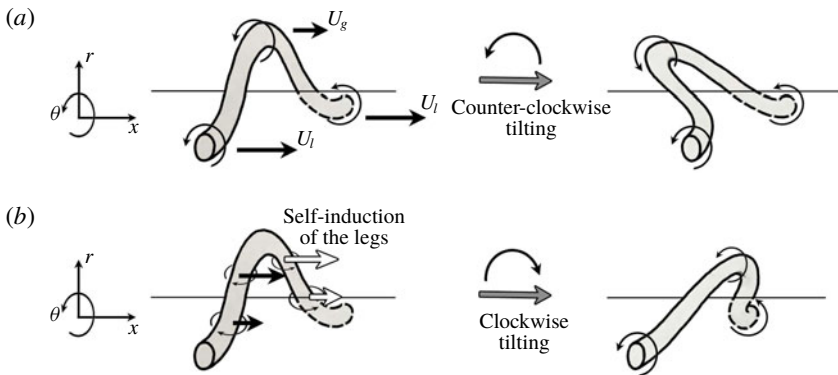
FIGURE 31. Opposite tilting effects: (a) upstream tilting of a transverse hairpin by the mean shear; (b) downstream tilting of a transverse hairpin by the hairpin’s self-induction.
