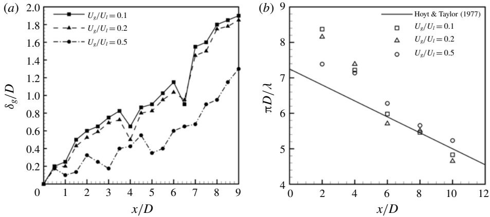
FIGURE 7. The growth of gas boundary layer thickness ( \delta_g ) along the axis (a); and comparison of the dimensionless wavenumber, \pi D/\lambda , obtained from the simulations, with the experimental data of Hoyt & Taylor (1977) (b).
