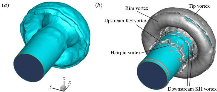
FIGURE 11. (Colour online) Liquid-jet surface near the cap (a); and vortices indicated by \lambda_2 = -10^{11} \text{ s}^{-2} isosurface (b), at t^* = 3.0 in case 2.
