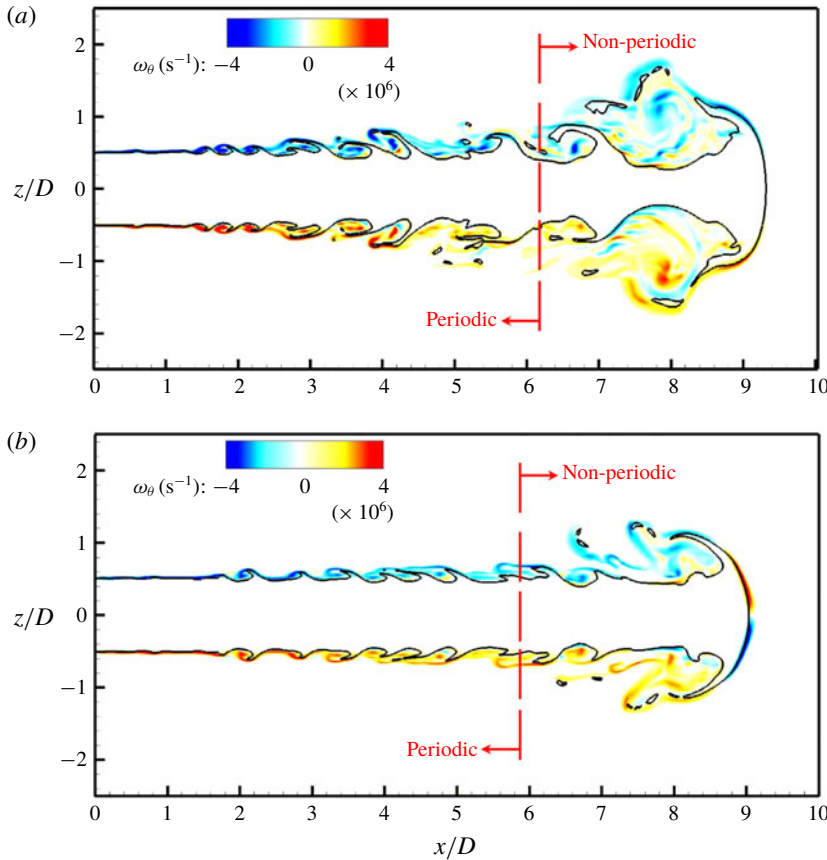
FIGURE 28. (Colour online) The liquid jet snapshots at t^* = 10.0 on a slice cutting through y = 0 ; case 1 (a), and case 3 (b).
