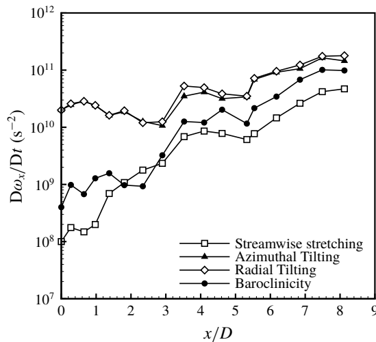
FIGURE 37. Contributions of streamwise vortex stretching, azimuthal vortex tilting, radial vortex tilting and baroclinicity to the generation of \omega_x at the jet surface for case 4; t^* = 11.5 .
