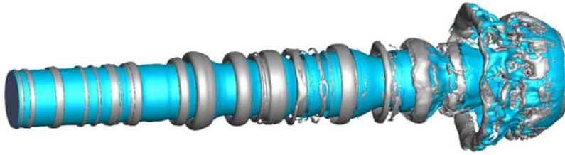
FIGURE 21. (Colour online) The vortex structures in case 3 at t^* = 11.25 (same time as in figure 9c).
