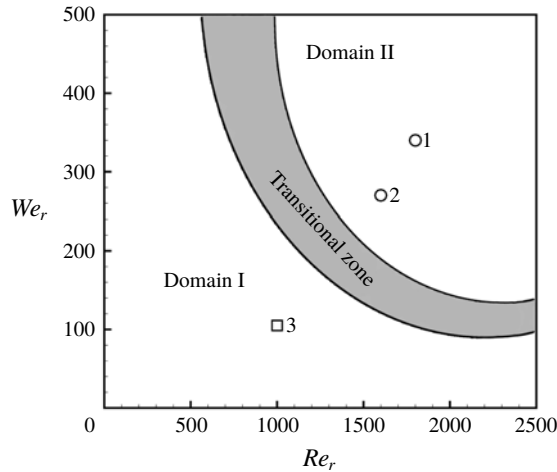
FIGURE 22. Identification of domains I and II on a We_r – Re_r diagram. The case numbers are indicated by the symbols. The approximate transitional zone has been denoted by the grey stripe.
