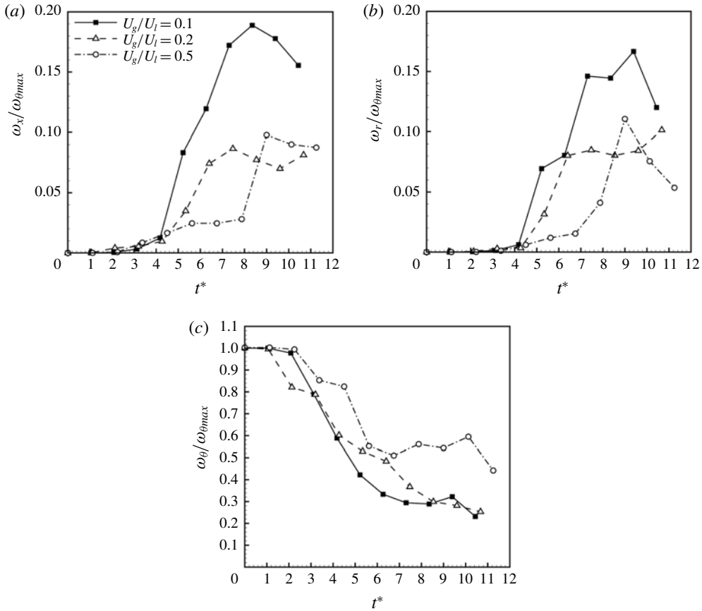
FIGURE 23. Kinematic variation of the normalized \omega_x (a); \omega_r (b); and \omega_{\theta} (c) for different velocity ratios.
