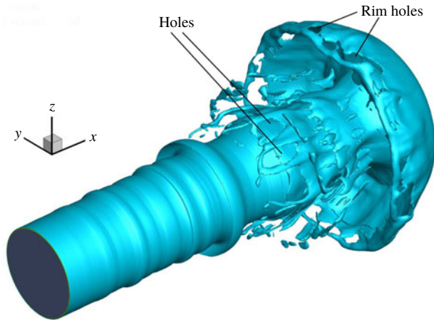
FIGURE 18. (Colour online) Liquid-jet surface at t^* = 5.5 in case 1.
