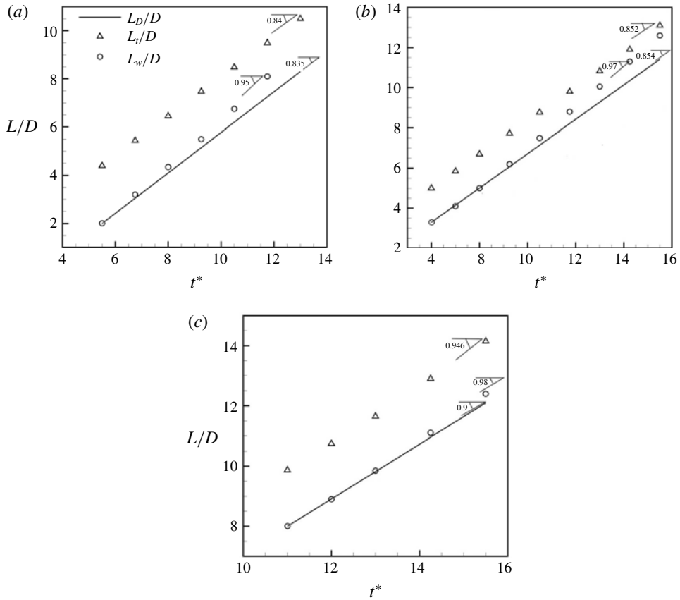
FIGURE 8. Temporal plot of L_t/D and L_w/D for case 1, \hat{U} = 0.1 (a); case 2, \hat{U} = 0.2 (b); and case 3, \hat{U} = 0.5 (c). The solid line indicates simple convection with Dimotakis velocity.
