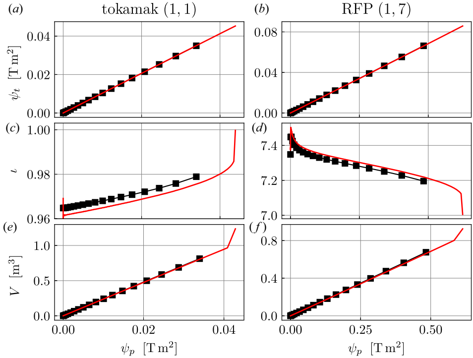
FIGURE 4. (a,b) Toroidal flux, (c,d) \nu and (e,f) volume as a function of the poloidal flux for (a,c,e) a (1,1) tokamak island and (b,d,f) a (1,7) RFP island, for the approaches of § 3 (red lines) and § 4 (black).
