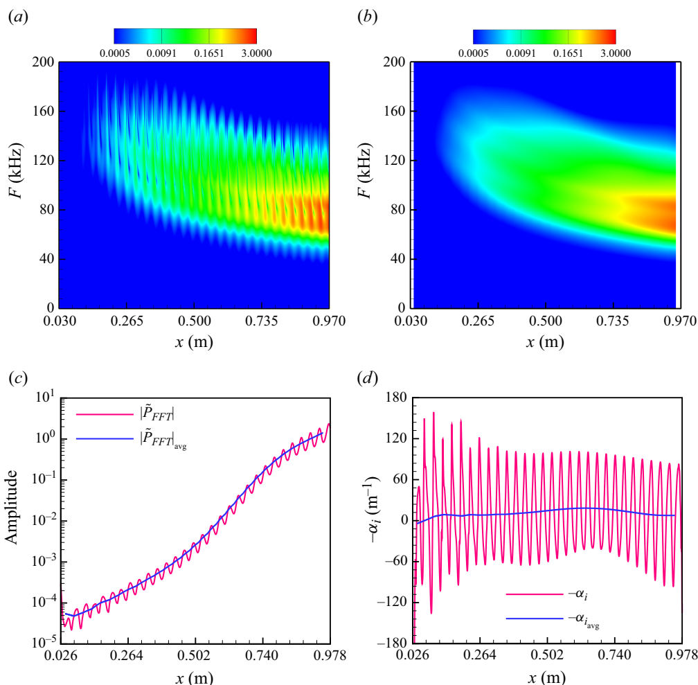
Figure 27. Fourier-transformed disturbance pressure amplitude for the rough-wall case W4A2 (a) before and (b) after averaging over each roughness wavelength. (c) Disturbance wall-pressure amplitude and (d) spatial growth rate extracted at F = 68 kHz, showing the actual and the roughness-averaged values along the surface.
