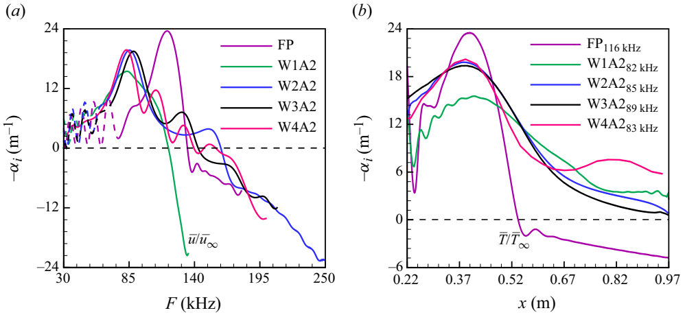
Figure 22. (a) Comparison of the averaged growth rate extracted at x = 0.4 m for the four wavelength-varying cases compared with the smooth-wall case as a function of the frequency. (b) Comparison of amplification rates along the wall corresponding to the frequencies leading to the maximum instability growth rate in (a).
