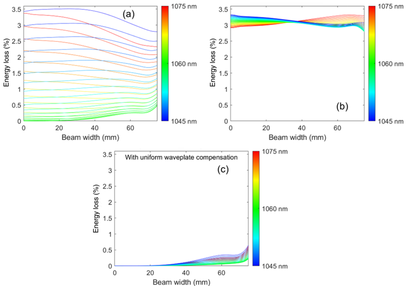
Figure 7. Wavelength dependence of depolarization as a function of beam width for wavelengths ranging from 1045 to 1075 nm at a 30 mrad multiplexing angle. (a) Both heads contain a right-handed QR. (b) Opposite-handed QRs in the two heads. (c) Same case as (b) with additional uniform waveplates for compensation.
