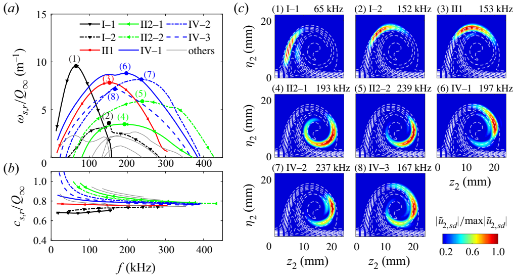
Figure 20. (a) Growth rates and (b) phase velocities of secondary instability modes at s = 1.0 m in the TCNE benchmark case, as well as (c) contours of their normalized streamwise ( s_2 ) velocity amplitudes of the most unstable one. The white dotted lines are the contours of the base streamwise velocity as in figure 17(b).
