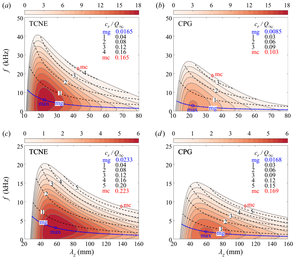
Figure 8. Growth rate contours (-\alpha_i) [ \text{m}^{-1} ] with frequencies and spanwise wavelengths: (a) TCNE and s = 0.2\text{ m} , (b) CPG and s = 0.2\text{ m} , (c) TCNE and s = 0.8\text{ m} and (d) CPG and s = 0.8\text{ m} . The contours of phase velocities are also plotted as dashed lines. The level in red labelled ‘mc’ is the maximum c_r/Q_\infty and the one in blue labelled ‘mg’ is the value of the most unstable mode.
