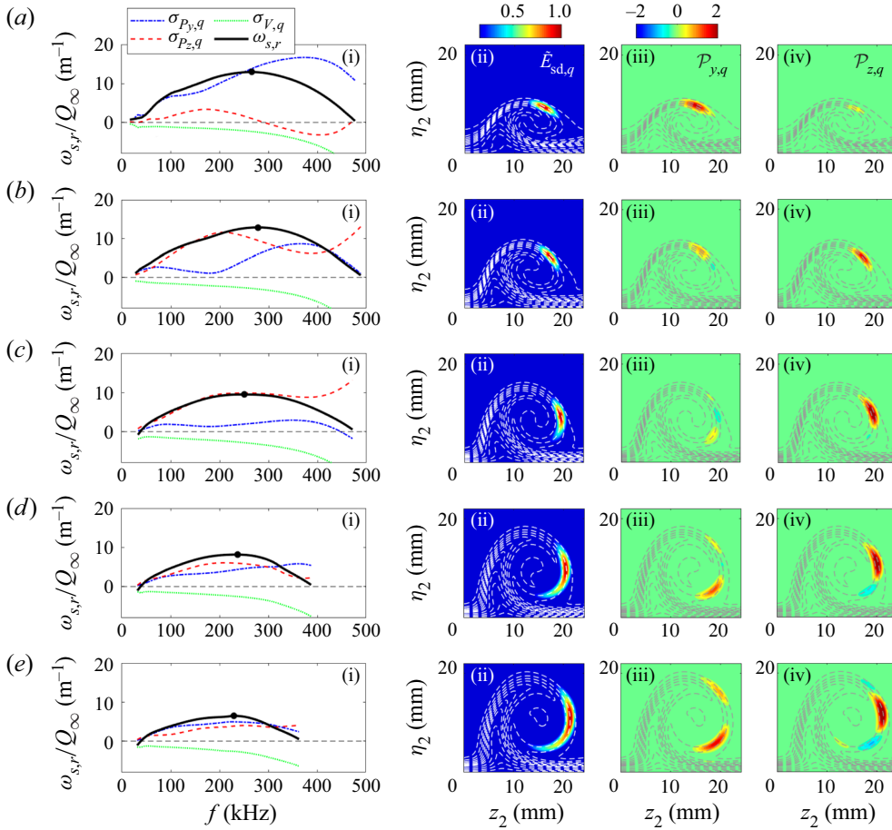
Figure 21. Streamwise development of the type-IV-2 mode at s of (a) 0.70 m, (b) 0.80 m, (c) 0.90 m, (d) 1.00 m and (e) 1.10 m. (i) The growth rate decomposition, and (ii)–(iv) the contours of the normalized disturbance energy, wall-normal and spanwise production terms, respectively.
