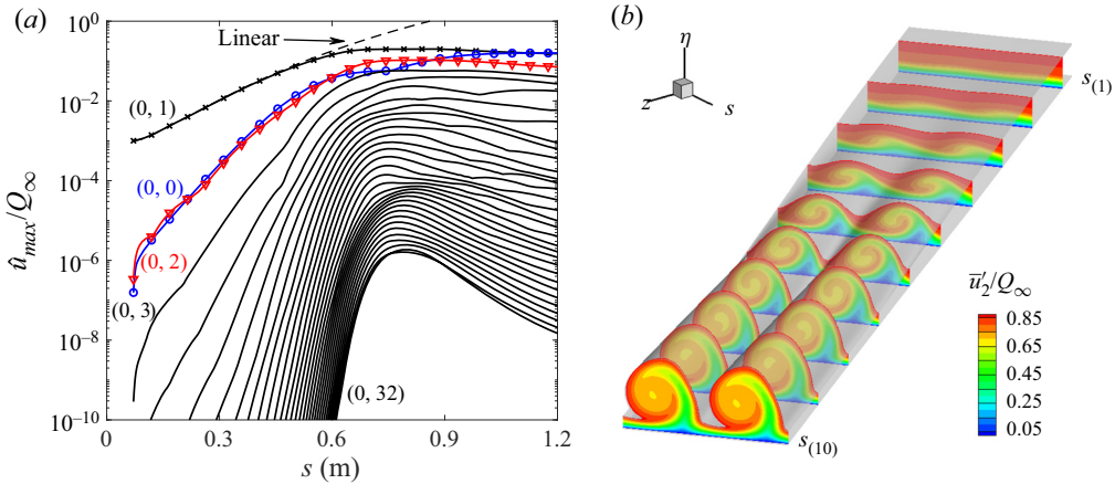
Figure 17. Streamwise development of (a) mode amplitudes and (b) contours of \bar{u}'_2 in the z_2 - \eta_2 plane. Note that the contours in (b) are originally plotted in the (s_2 - \eta_2 - z_2) coordinates (compressed in the s_2 direction for clarity) and then transformed back to the (s - \eta - z) coordinates to be consistent with (a). Therefore, the streamwise location in (b) is based on s , and the ten stations displayed are evenly distributed ranging from s_{(1)} = 0.33 m to s_{(10)} = 1.20 m.
