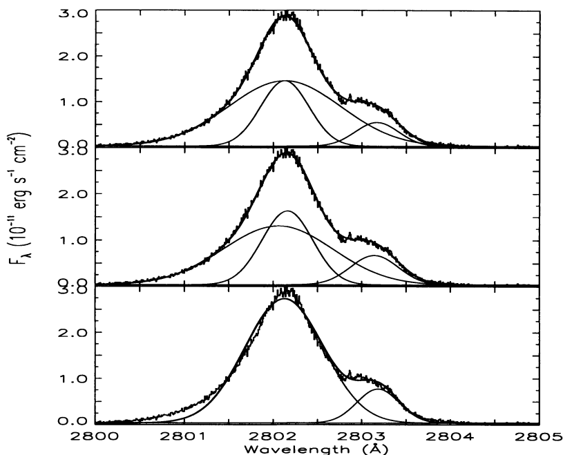
Figure 1. Evolution of gaussian fits to the Mg II h-line. In the bottom panel a single component is used for the K and G star, respectively. A third component was added in the middle panel. A broad gaussian near the K star velocity is favored. The top panel represents an optimum fit with the broad and narrow K-star gaussian being fixed to the same position.
