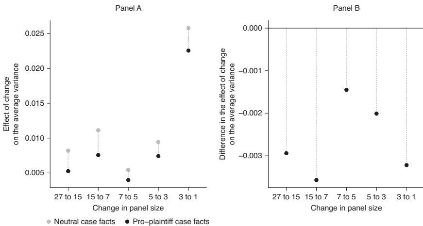
Figure 4. Comparative statics: The location of the case facts. Notes: This figure shows the predicted effect of chamber size ( s ) on the average variance of the probability that the plaintiff wins ( \bar{V} ), conditional on the mean of the case facts distribution ( \mu_{fc} ). Panel A shows the effect of various changes in chamber size when case facts are neutral ( \mu_{fc} = 0 ) and when case facts favor the plaintiff ( \mu_{fc} = 1 ). Panel B shows the change in each effect caused by increasing the mean.
