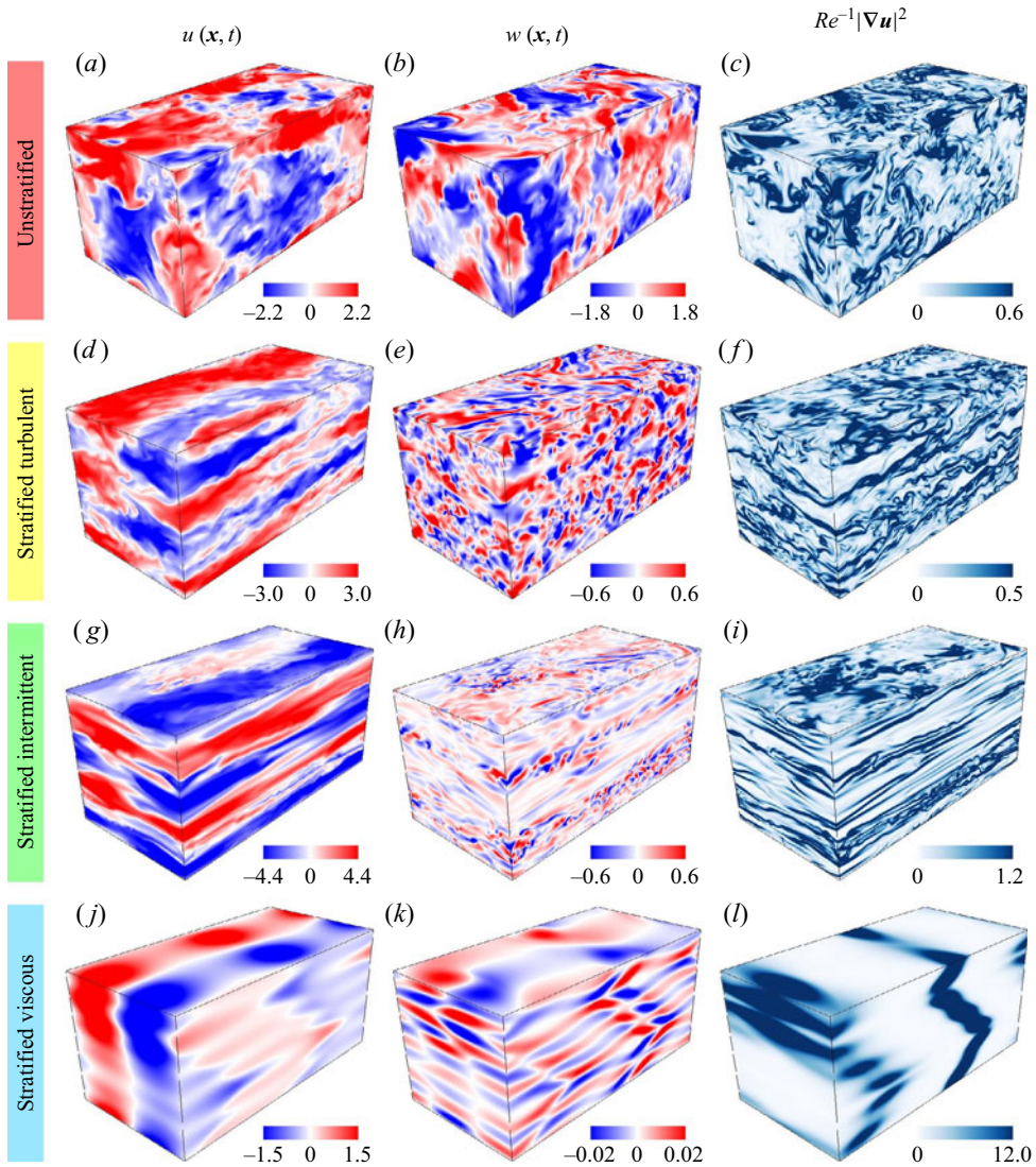
FIGURE 6. Snapshots of the streamwise velocity ( a, d, g, j ), vertical velocity ( b, e, h, k ) and local viscous dissipation rate ( c, f, i, l ) during the statistically stationary states of DNSs with Pe = 0.1 and: ( a-c ) Re = 300 , B = 1 ; ( d-f ) Re = 300 , B = 100 ; ( g-i ) Re = 300 , B = 10\,000 ; ( j-l ) Re = 50 , B = 100\,000 . Each of these examples are characteristic of a particular regime, listed on the left.
