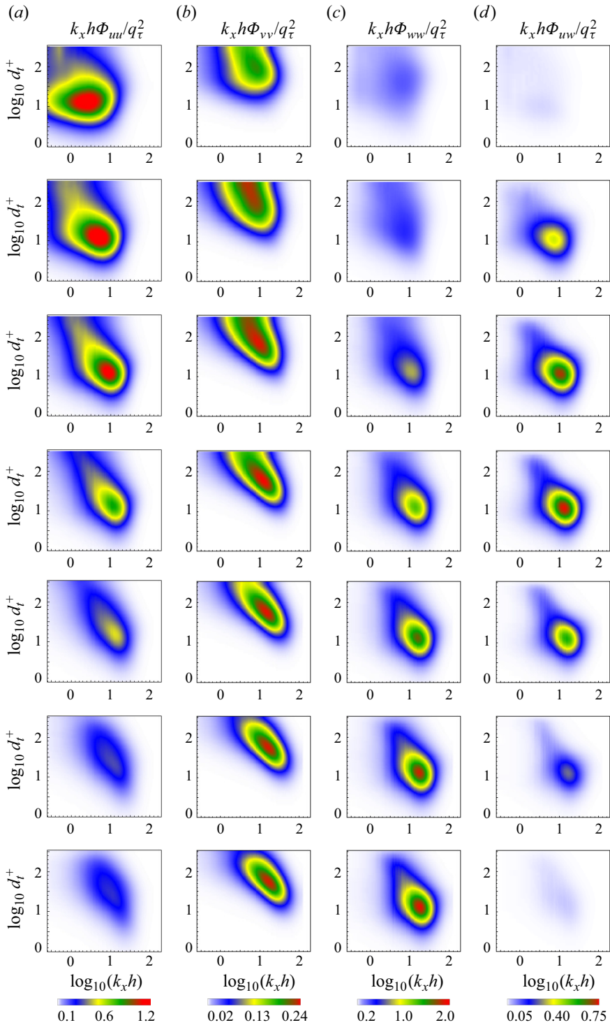
Figure 16. Contours of k_x -premultiplied 1-D spectra for OCP flow ( \phi = 90^\circ ): (a) k_x h \Phi_{uu}/q_\tau^2 , (b) k_x h \Phi_{vv}/q_\tau^2 , (c) k_x h \Phi_{ww}/q_\tau^2 , (d) k_x h \Phi_{uw}/q_\tau^2 . From top to bottom: \theta from 0^\circ to \theta = 90^\circ with increments of 15^\circ .
