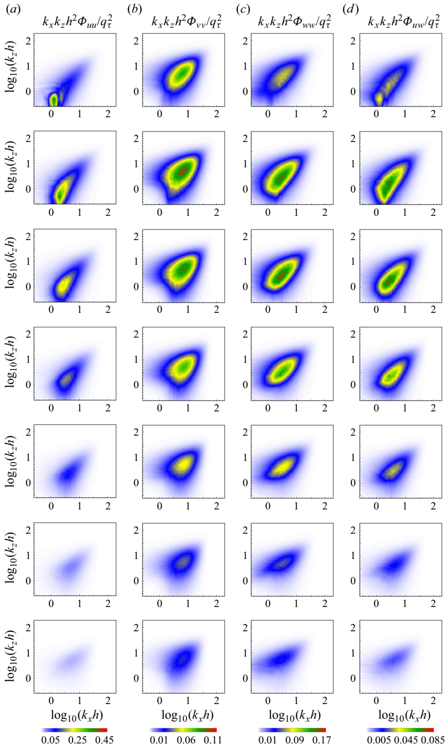
Figure 19. Contours of the k_x - and k_z -premultiplied 2-D spectra on the centre line y = 0 : (a) k_x k_z h^2 \Phi_{uu} / q_\tau^2 , (b) k_x k_z h^2 \Phi_{vv} / q_\tau^2 , (c) k_x k_z h^2 \Phi_{ww} / q_\tau^2 , (d) k_x k_z h^2 \Phi_{uw} / q_\tau^2 . From top to bottom: \theta from 0^\circ to \theta = 90^\circ with increments of 15^\circ .
