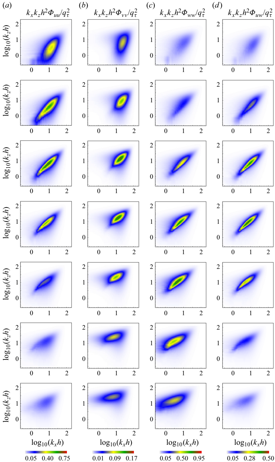
Figure 18. Contours of k_x - and k_z -premultiplied two-dimensional (2-D) spectra at around a_t^+ = 30 : (a) k_x k_z h^2 \Phi_{uu}/q_\tau^2 , (b) k_x k_z h^2 \Phi_{vv}/q_\tau^2 , (c) k_x k_z h^2 \Phi_{ww}/q_\tau^2 , (d) k_x k_z h^2 \Phi_{uw}/q_\tau^2 . From top to bottom: \theta from 0^\circ to \theta = 90^\circ with increments of 15^\circ .
