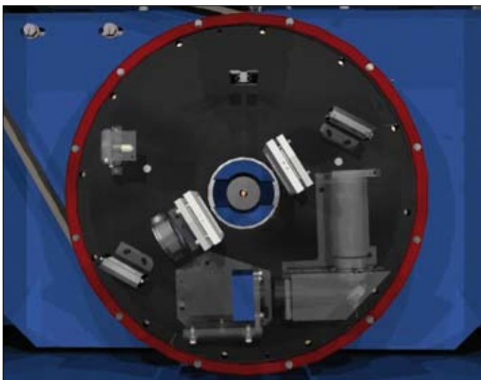
Siroll Orbis+: Optical unit with LED light source and camera. Source: Siemens
