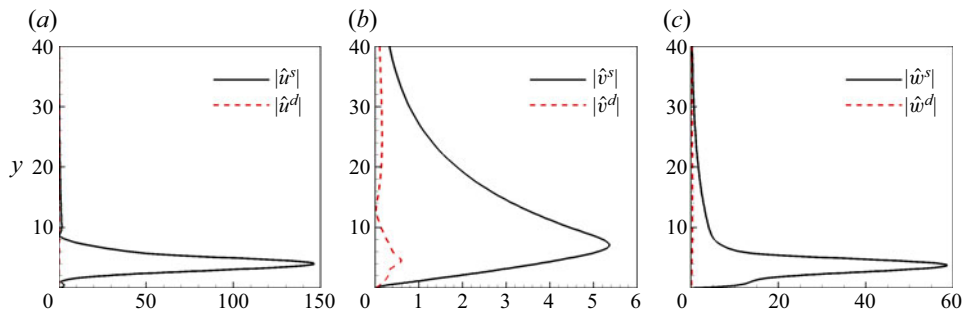
Figure 6. Mode shapes of the solenoidal and dilatational parts of (a) streamwise velocity ( \hat{u} ), (b) wall-normal velocity ( \hat{v} ) and (c) spanwise velocity ( \hat{w} ), for the most unstable first mode at M = 3.0 .
