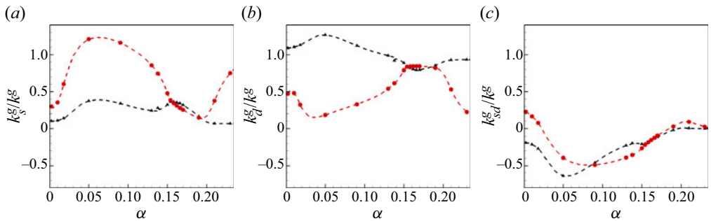
Figure 16. (a) Solenoidal ( k_s^g ), (b) dilatational ( k_d^g ) and (c) covariance ( k_{sd}^g ) components of kinetic energy for the fast and slow modes at M = 6 . Black and red lines with symbols correspond to the fast and slow modes, respectively.
