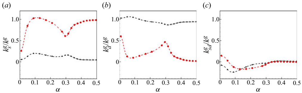
Figure 15. (a) Solenoidal ( k_s^g ), (b) dilatational ( k_d^g ) and (c) covariance ( k_{sd}^g ) components of kinetic energy for the fast and slow modes at M = 4 . Black and red lines with symbols correspond to the fast and slow modes, respectively.
