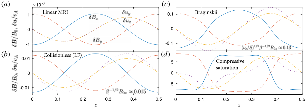
FIGURE 2. The structure of a kinetic MRI mode evolving in a vertical background field B_{0z} in various regimes, as computed from the 1-D LF model (with \nu_c \neq 0 in panel c ). We take \beta_0 = 337 in a domain with \Omega L_z/c_s = 1 , such that the peak of the MRI dispersion relation (i.e. the maximum \gamma ) is at k = 2 \times 2\pi/L_z (each panel shows only half of a scale height). Each plot illustrates \delta B_x (blue solid line), \delta B_y (red dashed line), \delta u_x (yellow dot-dashed line) and \delta u_y (purple dotted line). The various panels show: (a) the linear KMRI mode (this is the initial conditions for each simulation), which is identical in structure to an MHD MRI mode at these parameters; (b) the collisionless MRI mode when \Delta p reaches the mirror limit ( \delta B \sim \beta^{-1/2} B_{0z} \approx 0.015 ), which remains very nearly sinusoidal because the heat fluxes make \Delta p spatially uniform; (c) a mode in the high-collisionality Braginskii regime (with \nu_c/S = \beta_0^{3/4} ) when \Delta p reaches the mirror limit (at \delta B \sim (\nu_c/S)^{1/2} \beta^{-1/2} B_{0z} \approx 0.13 ), which is non-sinusoidal because of the O(1) spatial variation in \Delta p ; (d) the MRI mode at very large amplitudes, when compressibility becomes important. The structure of this final compressible stage of evolution is the same across all models, including standard (collisional) MHD.
