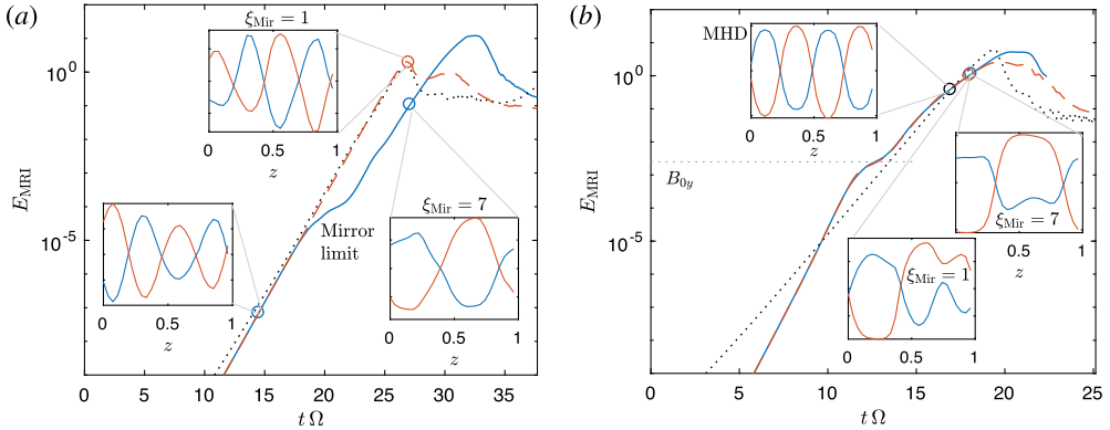
FIGURE 6. Energy of the MRI perturbation, E_{\text{MRI}} = \int dz (\rho \delta u^2/2 + \delta B^2/8\pi) , as a function of time for a set of 3-D ZEUS simulations at \beta_0 = 400 . We compare the evolution of the LF model (2.1)–(2.7) with mirror limiter \Delta = 7/\beta as used in S06 (blue solid lines), the LF model with mirror limiter \Delta = 1/\beta (red dashed lines) and standard MHD (black dotted lines). The insets show the vertical mode structure ( \delta B_x , blue; \delta B_y , red) at the times indicated by the circles. Panel (a) shows the case with a purely vertical background magnetic field ( B_{0y} = 0 ). This illustrates how an artificially high mirror limit ( \Delta = 7/\beta ; blue solid line) causes the mode to move to longer wavelengths after it reaches the mirror limit at t \approx 17 , which subsequently causes the mode to reach a very large amplitude before saturation. Panel (b) shows simulations with an azimuthal background magnetic field ( B_{0y} = B_{0z} ; the dotted line shows the energy of B_{0y} ); in this case, all three modes saturate into turbulence at similar amplitudes. Given the relatively disordered mode structure in the kinetic runs (the insets compare the late-time structures of all three cases, as labelled), this behaviour is consistent with the idea that there are not major differences between the parasitic modes' properties in the kinetic (LF) model and MHD (see text for further discussion). Note that the time scale of the MHD case in panel (b) has been shifted to the left, so that all three modes reach saturation amplitudes at a similar time (the linear growth of the KMRI mode is faster, see figure 1).
