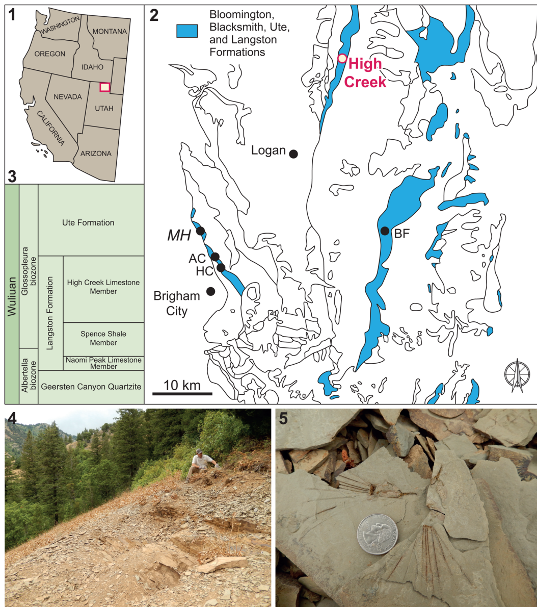
Figure 2. Locality information. (1) Map of western United States with indication of the area exposing the Langston Formation. (2) Enlargement of the red rectangular area in (1). (3) Simplified stratigraphy of the Langston Formation. (4) Quarry rich in echinoderms in the Langston Formation at High Creek locality, Utah. (5) Moldic preservation of undescribed eocrinoid from the productive horizon. (1–3) From Kimmig et al. (2019).
