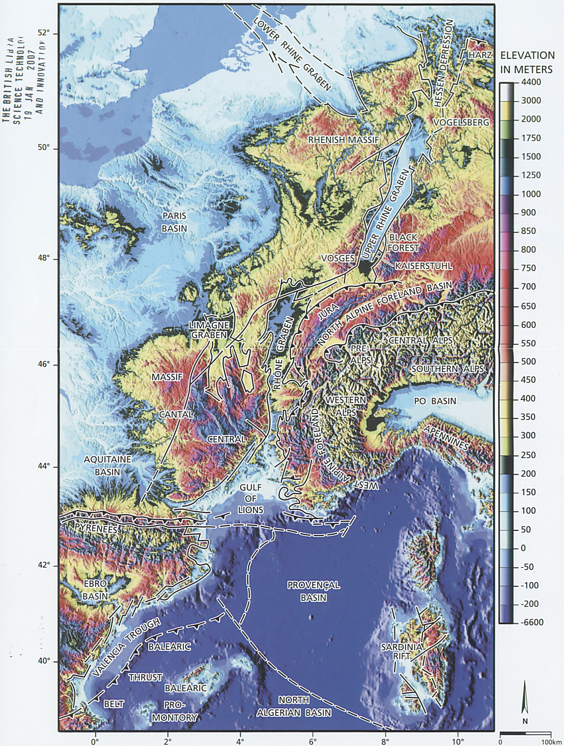
Encl. 1. Digital elevation map of the European Cenozoic Rift System (Lower Rhine Graben and Hessen Depression to Valencia Trough, Massif Central grabens) and its adjoining areas
