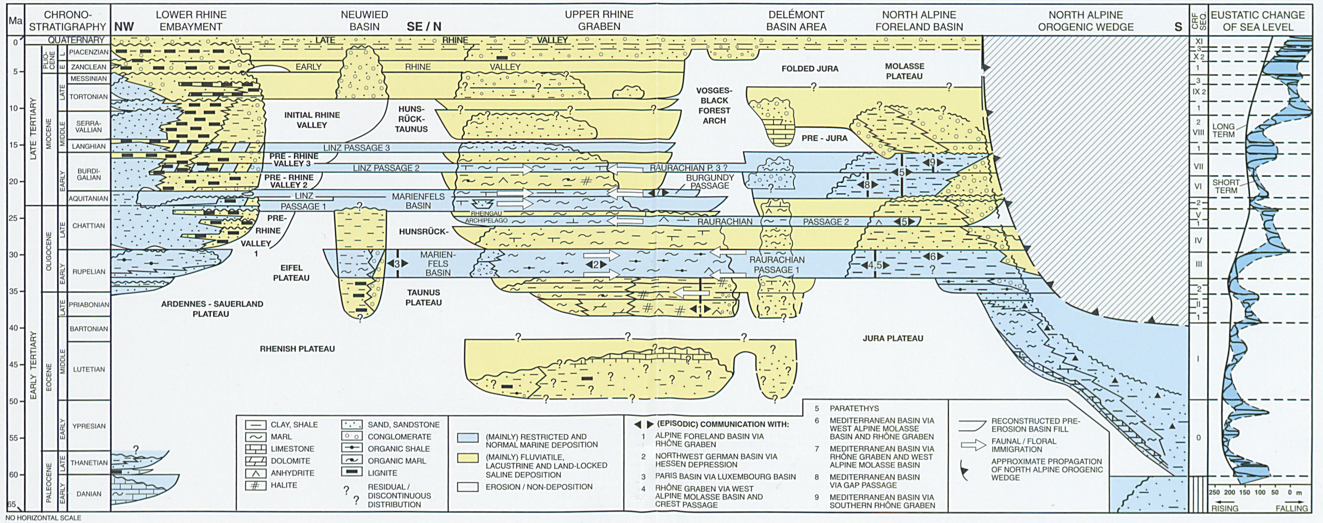
Encl. 5. Sequence stratigraphic interpretation of the Northern European Cenozoic Rift Segment (Lower Rhine Embankment to Upper Rhine Graben) and North Alpine Foreland Basin (central part). After Sissingh (2003b)
