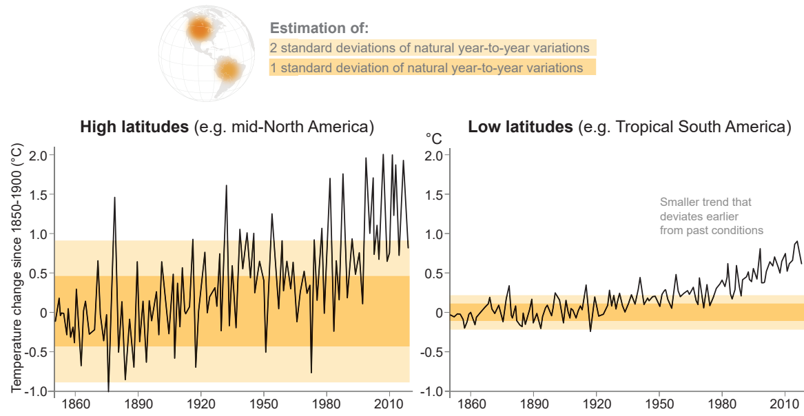
FAQ 1.2, Figure 1 | Observed variations in regional temperatures since 1850 (data from Berkeley Earth). Regions in high latitudes, such as mid-North America (40°N–64°N, 140°W–60°W, left ), have warmed by a larger amount than regions at lower latitudes, such as tropical South America (10°S–10°N, 84°W–16°W, right ), but the natural variations are also much larger at high latitudes (darker and lighter shading represents 1 and 2 standard deviations, respectively, of natural year-to-year variations). The signal of observed temperature change emerged earlier in tropical South America than mid-North America even though the changes were of a smaller magnitude. (Note that those regions were chosen because of the longer length of their observational record; see Figure 1.14 for more regions).
