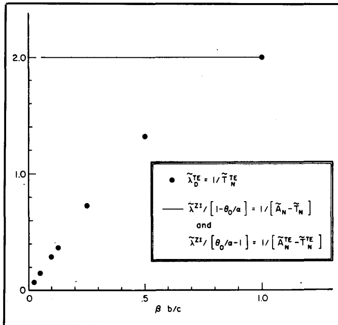
Figure 3. Aeroelastic coefficients required for zero wall interference; divergence aeroelastic coefficient shown for reference.
