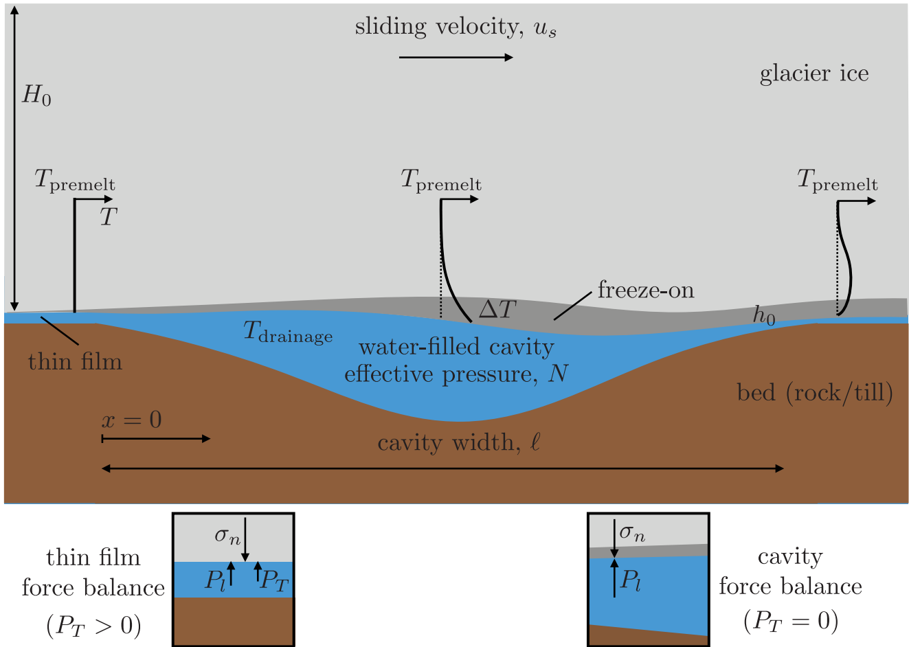
Fig. 1. Schematic of a representative cavity, with uniform liquid temperature T_{\text{drainage}} = T_{\text{pre-melt}} + \Delta T , connected to pre-melted films that separate the bounding rock/till interface from the overlying glacier ice. Representative temperature profiles are shown (left to right): (i) at the upstream side of the cavity prior to unloading (constant at T_{\text{pre-melt}} ), (ii) midway over the cavity with a conductive profile promoting freeze-on (decaying from T_{\text{drainage}} to T_{\text{pre-melt}} far above the bed), and (iii) at the downstream side of the cavity after the interface temperature has returned to T_{\text{pre-melt}} and melting has commenced (note the dissipating thermal wave above the bed). Note that the melt rate at (iii) is lower than the freezing rate at (ii), promoting net freeze-on as ice flows across the schematic. Lower schematics show the force balance in the pre-melted film (left; P_T > 0 ) and in the cavity (right; P_T = 0 ).
