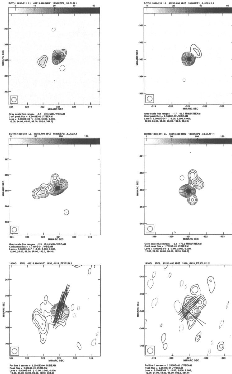
Figure 1. Multi-epoch 43 GHz VLBA maps of 1830–211 NE (left) and 1830–211 SW (right). The epoch of observation increases from top to bottom. Contours are spaced by factors of two in brightness, with the lowest at three times the rms noise ( \sim 0.5 mJy per beam) of the 19 Jan 1997 maps. The FWHM of the circular restoring beam is 0.33 mas.
