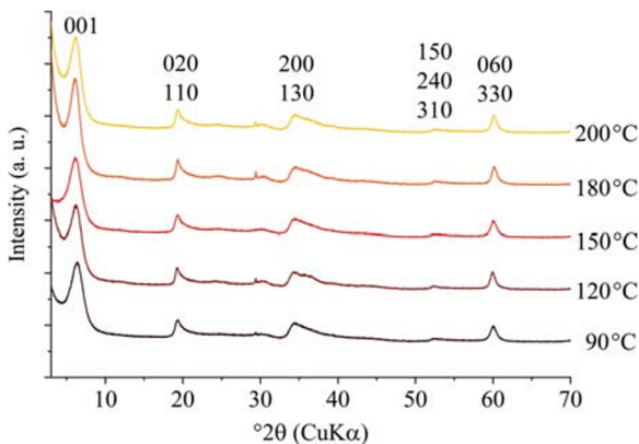
Fig. 4. Powder XRD pattern of synthetic saponite with indexed diffraction planes at various temperatures. d_{001} = 1.5\text{ nm} and d_{060} = 0.154\text{ nm}
