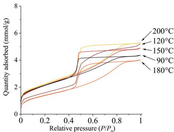
Fig. 9. Isotherms of nitrogen adsorption and desorption for saponites synthesized at various temperatures
