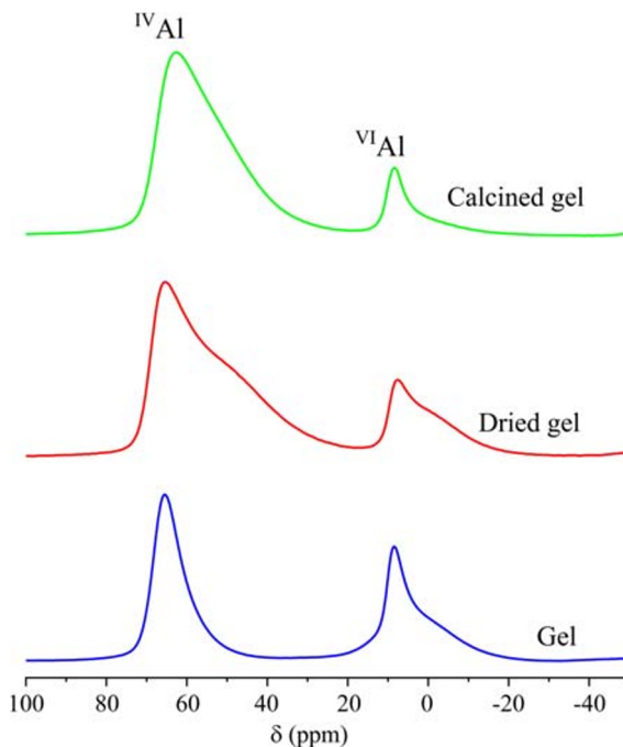
Fig. 3. ^{27}\text{Al} MAS NMR spectra of samples synthesized at 200°C with various precursor preparation methods. ^{\text{VI}}\text{Al} and ^{\text{IV}}\text{Al} corresponds to
