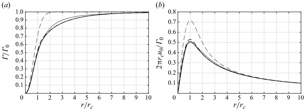
Figure 1. Circulation (a) and induced velocity (b) profiles for various wake vortex models: single scale models, BH (thin solid) and LO (thin dash); two-scale models for the case r_c/b_0 = 0.050 , P (dash) and PW (solid).
