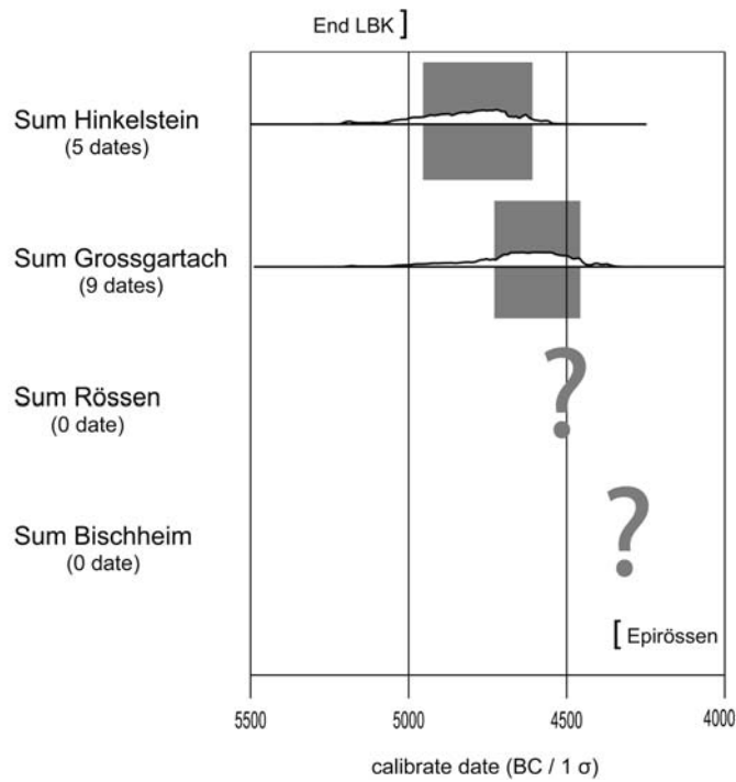
Figure 7 ^{14}\text{C} dating on bones of Hinkelstein, Grossgartach, Rössen, and Bischheim. Sum of the probabilities calculated with the software OxCal 3.10.
