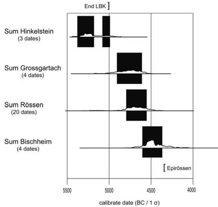
Figure 6 ^{14}\text{C} dating on charcoals of Hinkelstein, Grossgartach, Rössen, and Bischheim. Sum of the probabilities calculated with the software OxCal 3.10.
