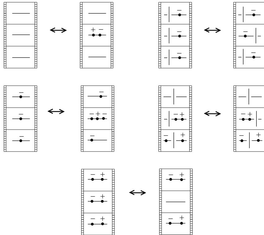
Figure 5: Additional movie moves for framed cobordisms.
