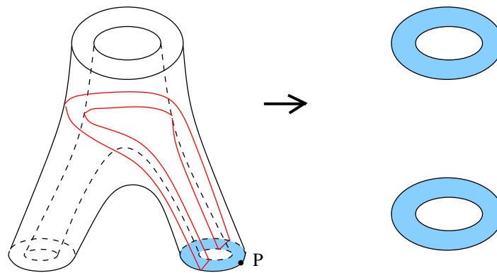
Figure 11: Commutativity of the diagrams of Figure 9. The filled regions are annuli of genus 1. Applying the neck cutting relation to the red line, and removing components of genus 2, we get one half of the two genus 1 annuli, shown on the right.
