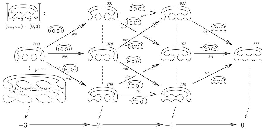
Figure 1: The cube of resolutions for the trefoil.
