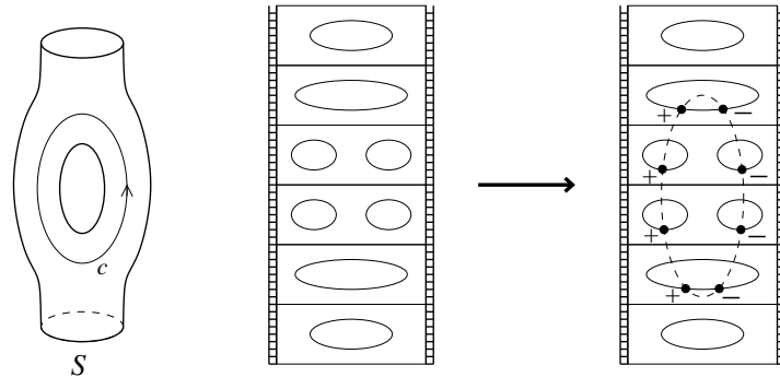
Figure 6: Inserting an oriented curve c into a movie.
