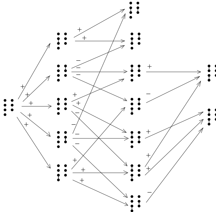
Figure 3: The graph \Gamma_{4,3} .
