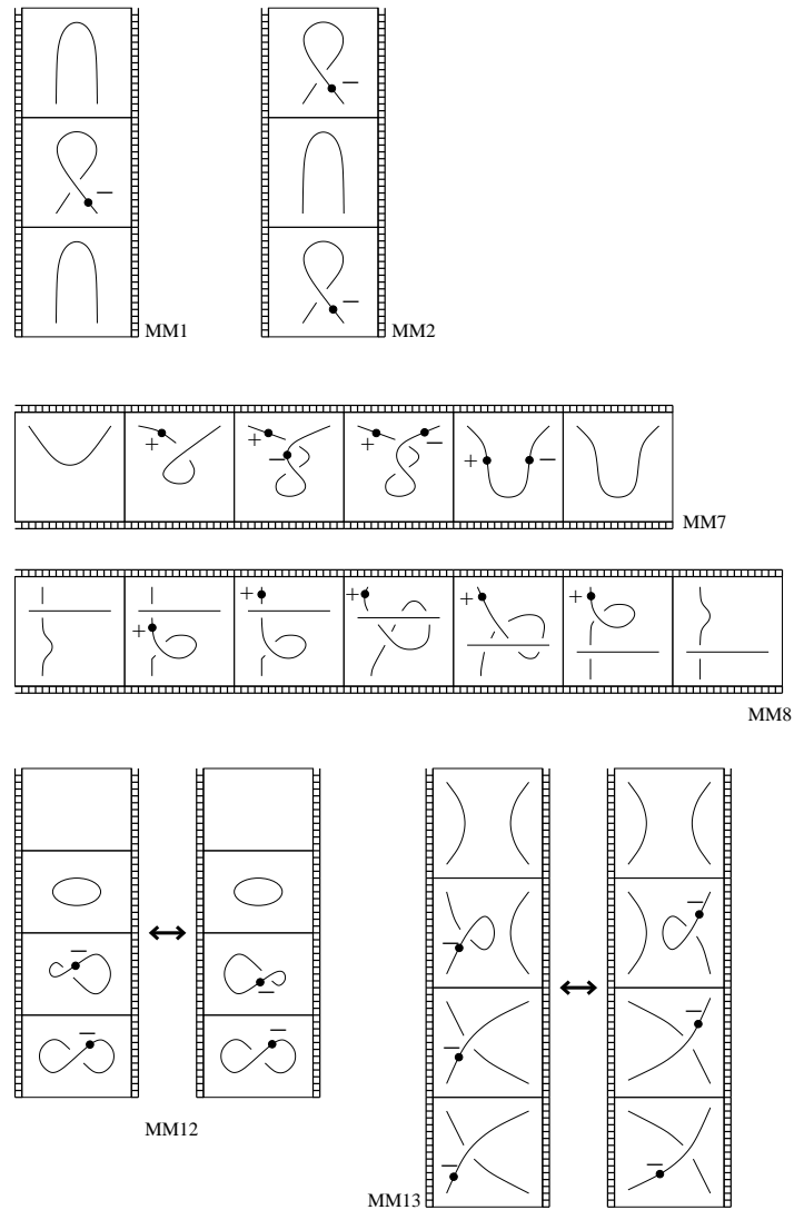
Figure 4: Modified Carter–Saito moves for framed cobordisms. These moves are obtained by inserting marked points into the original Carter–Saito moves, in such a way that each R1 move becomes an MR1 move. The modified moves MM3–MM6, MM9–MM11, MM14 and MM15 are not displayed because they are identical with the corresponding original Carter–Saito moves. When lifting an R1 move to an MR1 move, one has two possibilities where to insert the marked point (one can place the marked point on either of the two sides of the curl). Only one possibility is shown above.
