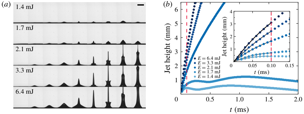
FIGURE 3. (Colour online) (a) Snapshots showing the evolution of the jet for sample 5 at z_f = 0.5 mm for various laser energies. The snapshots show the evolution of the jet for t = 0.0, 0.01, 0.02, 0.05, 0.1, 0.18, 0.33, 0.61, 1.1 and 2.0 ms. The scale bar corresponds to 2 mm. (b) The vertical extent of the jets versus time. The inset shows a zoom-in of the region for the early stage of ejection. The red dashed line demarcates the region t \leq 0.1 ms in which a quadratic fit is applied to extrapolate the jet velocity at t = 0 . See the supplementary movies for the examples shown here.
