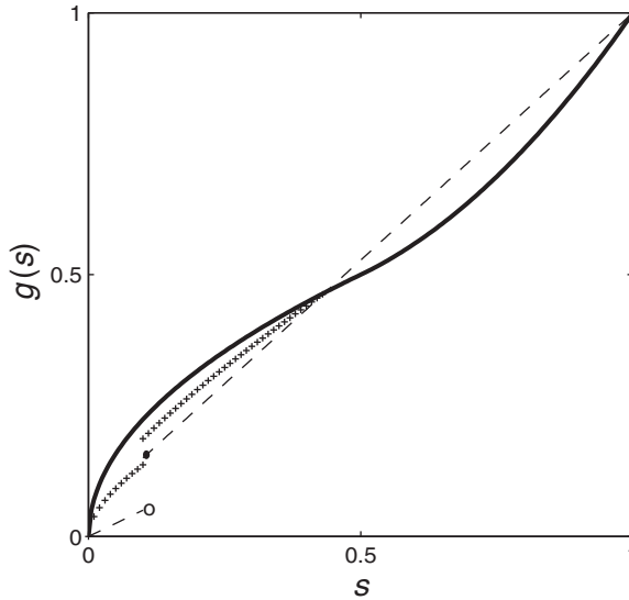
FIGURE 3: We graphically display the premium principle. The distortion function of the insurer is inverse-S shaped (the solid line) and the preferences of the reinsurer are given in (23), with \gamma = 0.9 and \beta = 0.1 (the dotted line). The optimal reinsurance contract is derived from Case 4.1, and is given by f^*(X) = (X - VaR_c(-X))_+ for c \approx 0.45 in this figure. The line of crosses is the distortion function that serves as a premium principle after bargaining with \alpha = 0.5 .
