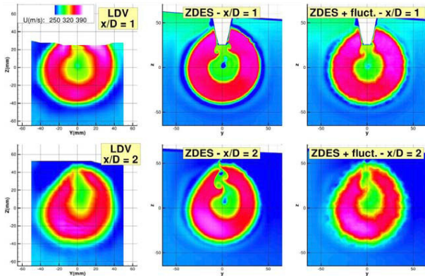
Fig. 10. Averaged velocity fields at x/D = 1 and 2. Left: LDV measurements – Middle: ZDES without RFG – Right: ZDES with RFG (Onera [34]).
