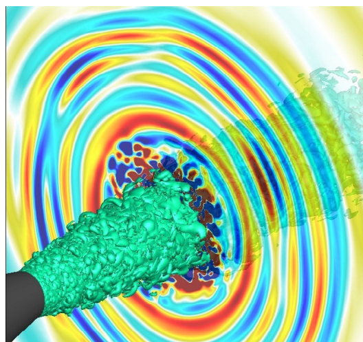
Fig. 15. Isothermal round jet LES elsA simulation: vorticity and dilatation fields (courtesy of Cerfacs).
