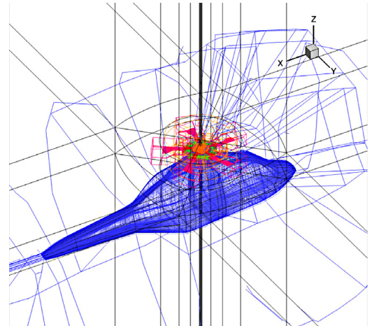
(a) Mesh of the helicopter with complete rotor head
