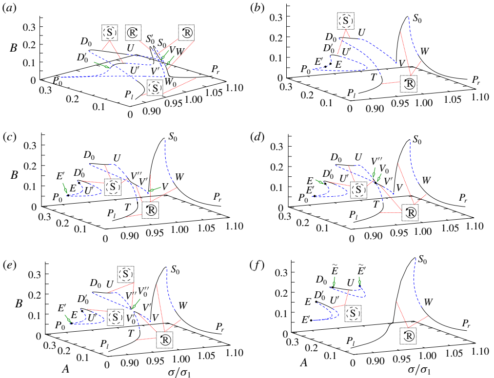
FIGURE 12. The same as in figures 10 and 11 but for \gamma = \pi/12 . The semi-axis ratio \delta_1 = 0.0 in (a) (harmonic oblique reciprocaton), \delta_1 = 0.6 (b), \delta_1 = 0.743 (c), \delta_1 = 0.744 (d), \delta_1 = 0.745 (e) and \delta_1 = 0.9 (f). The physical input data are taken from (3.30). The panels qualitatively repeat the wave-amplitude metamorphoses of the response curves in figures 10 and 11. An exception is the branch D'_0U'P_0D'_0 , which does not emerge from a single point as happened for \gamma = \pi/6 . The latter fact implies two (not one) stable nearly standing wave modes (points on D_0U and D'_0U' ) existing for all 0 \leq \delta_1 \leq 1 .
