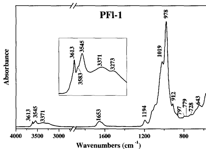
Figure 26. IR spectrum of PFI-1 palygorskite using the ATR technique. Insert: the OH-stretching region.
