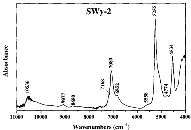
Figure 12. Diffuse-reflectance NIR spectrum of SWy-2 (montmorillonite).
