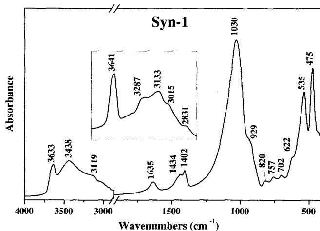
Figure 22. IR spectra of Syn-1 (mica-montmorillonite) using 0.5 mg sample/200 mg KBr for 4000–400 \text{cm}^{-1} . Insert: 2.0 mg sample/200 mg KBr, disk heated overnight at 150°C.
