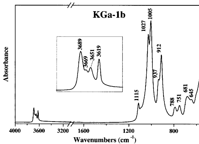
Figure 5. IR spectrum of KGa-1b (kaolinite) using the ATR technique. Insert: the OH-stretching region.
