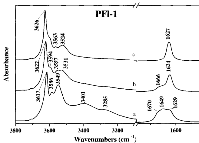
Figure 27. IR spectra of self-supporting film of PFI-1 palygorskite: (a) unheated, (b) heated at 180°C for 0.5 h; and (c) heated at 180°C for 1 h.
