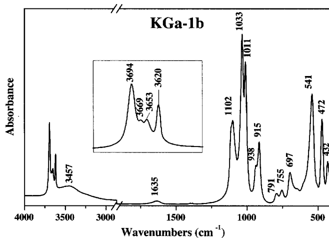
Figure 4. IR spectra of KGa-1b (kaolinite) using 0.5 mg sample/200 mg KBr for 4000–400 \text{cm}^{-1} . Insert: 2.0 mg sample/200 mg KBr, disk heated overnight at 150°C.
