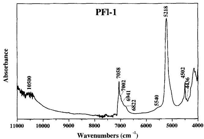
Figure 28. Diffuse-reflectance NIR spectrum of PFI-1 palygorskite.
