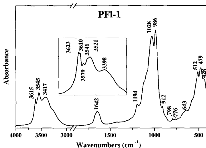
Figure 25. IR spectra of PFI-1 (palygorskite) using 0.5 mg sample/200 mg KBr for 4000–400 \text{cm}^{-1} . Insert: 2.0 mg sample/200 mg KBr, disk heated overnight at 150°C.
