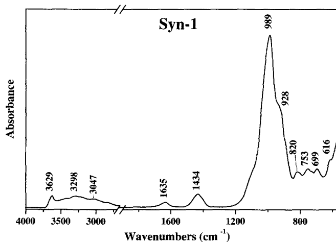
Figure 23. IR spectrum of Syn-1 (mica-montmorillonite) using the ATR technique.
