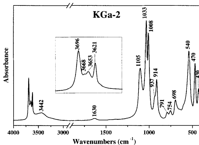
Figure 6. IR spectra of KGa-2 (kaolinite) using 0.5 mg sample/200 mg KBr for 4000–400 \text{cm}^{-1} . Insert: 2.0 mg sample/200 mg KBr, disk heated overnight at 150°C.
